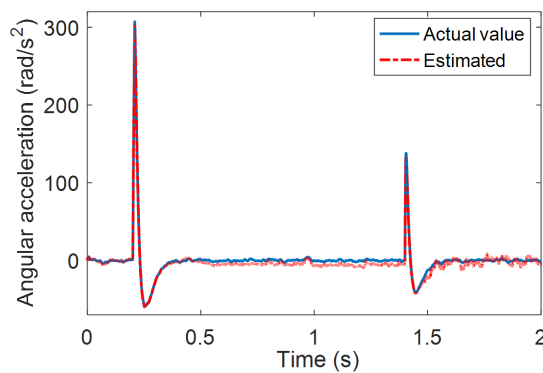
Fig. 16. The angular acceleration of actuator gear
