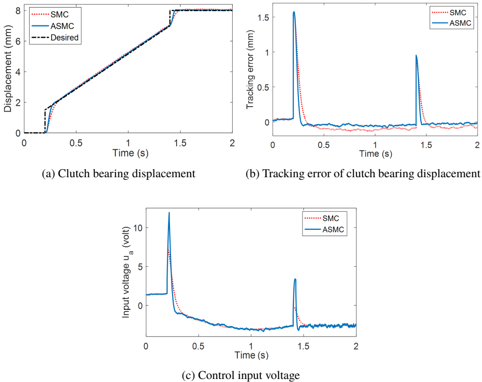
Fig. 17. Evaluation of SMC performance in comparison with the ASMC in the presence of 10% parameter uncertainties
