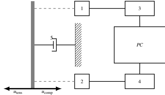
Fig. 3. Scheme of the measuring system used. 1 – displacement sensor, 2 – force sensor, 3, 4 – DAQ devices, 5 – investigated damper, u_{\text{tens}} – facing of tensioning of a specimen, u_{\text{comp}} – facing of compressing of a specimen
