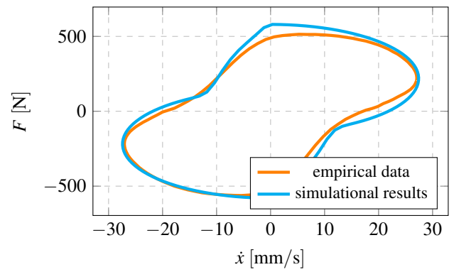
Fig. 14. Experimental hysteresis loop for p = 0.06 MPa; B-W model identified for the following parameters: a = 0.35, A = 6, \beta = 3, \gamma = -2, n = 4
