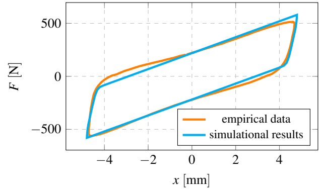
Fig. 13. Experimental hysteresis loop for p = 0.06 MPa; B-W model identified for the following parameters: a = 0.35, A = 6, \beta = 3, \gamma = -2, n = 4
