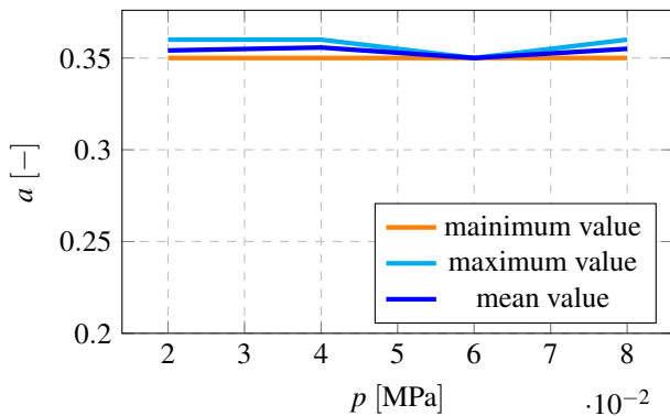
Fig. 18. Influence of underpressure on a parameter – the smallest RMS errors
