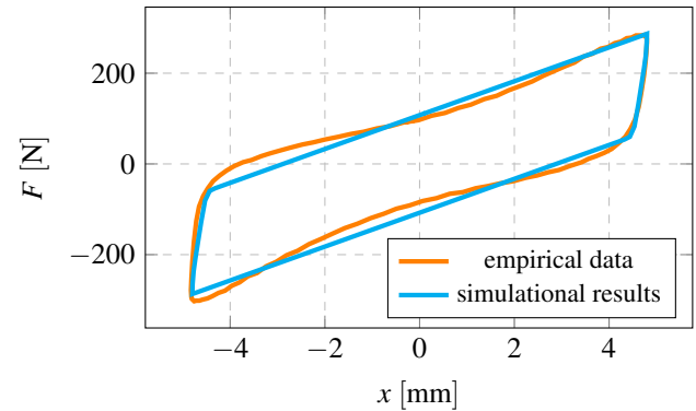
Fig. 9. Experimental hysteresis loop for p = 0.02 MPa; B-W model identified for the following parameters: a = 0.36, A = 9, \beta = 4, \gamma = -3, n = 5
