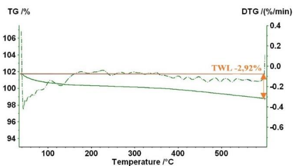
Fig.13. TG / DTG curve measured for sample no. 3 (after biodegradation process)
