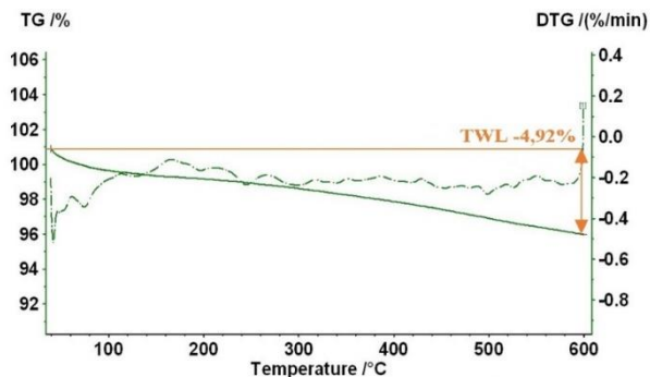
Fig. 3. TG / DTG curve measured for sample no. 1
