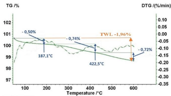
Fig. 10. TG / DTG curves measured for sample no. 8
