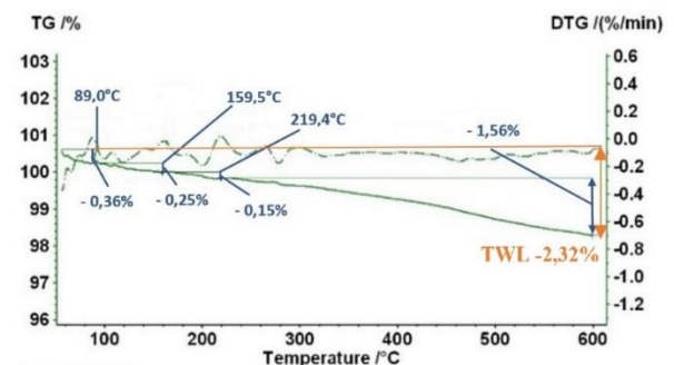
Fig. 6. TG / DTG curves measured for sample no. 4
