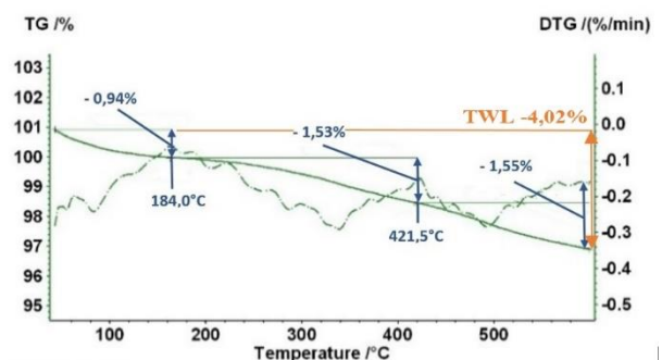
Fig. 8. TG / DTG curves measured for sample no. 6
