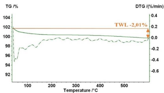
Fig.14. TG / DTG curve measured for sample no. 4 (after biodegradation process)
