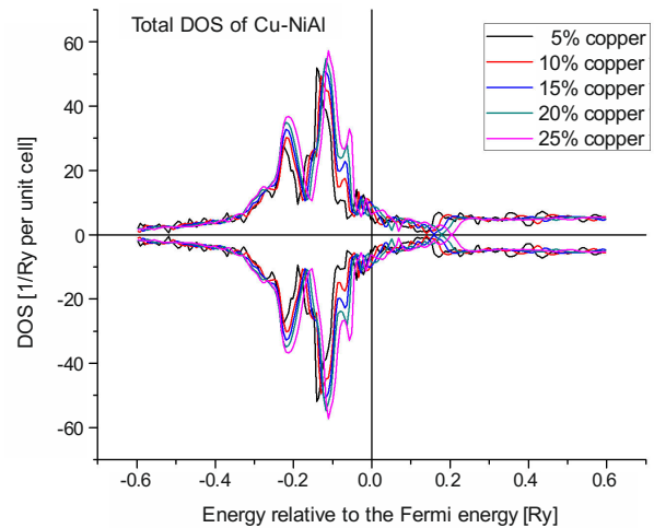
Fig. 4. Densities of states of different concentrations of Cu-doped NiAl where doping is in Al sites.
