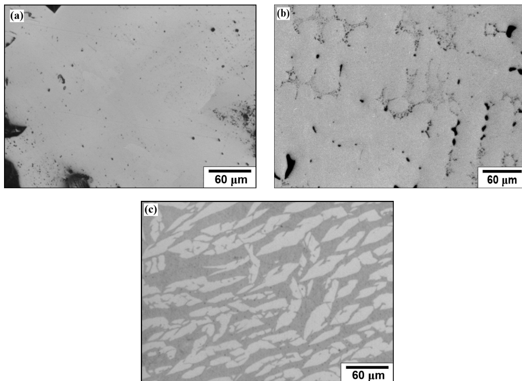
Fig. 2. Metallurgical microscope images of: NiAl 0.8 Cu 0.2 (a), NiAl 0.7 Cu 0.3 (b), and NiAl 0.6 Cu 0.4 (c).
