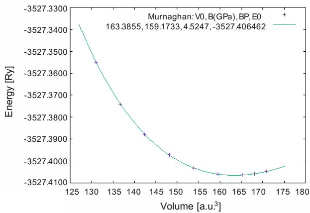
Fig. 3. Structure parameters optimization of a NiAl unit cell (Relaxation).
