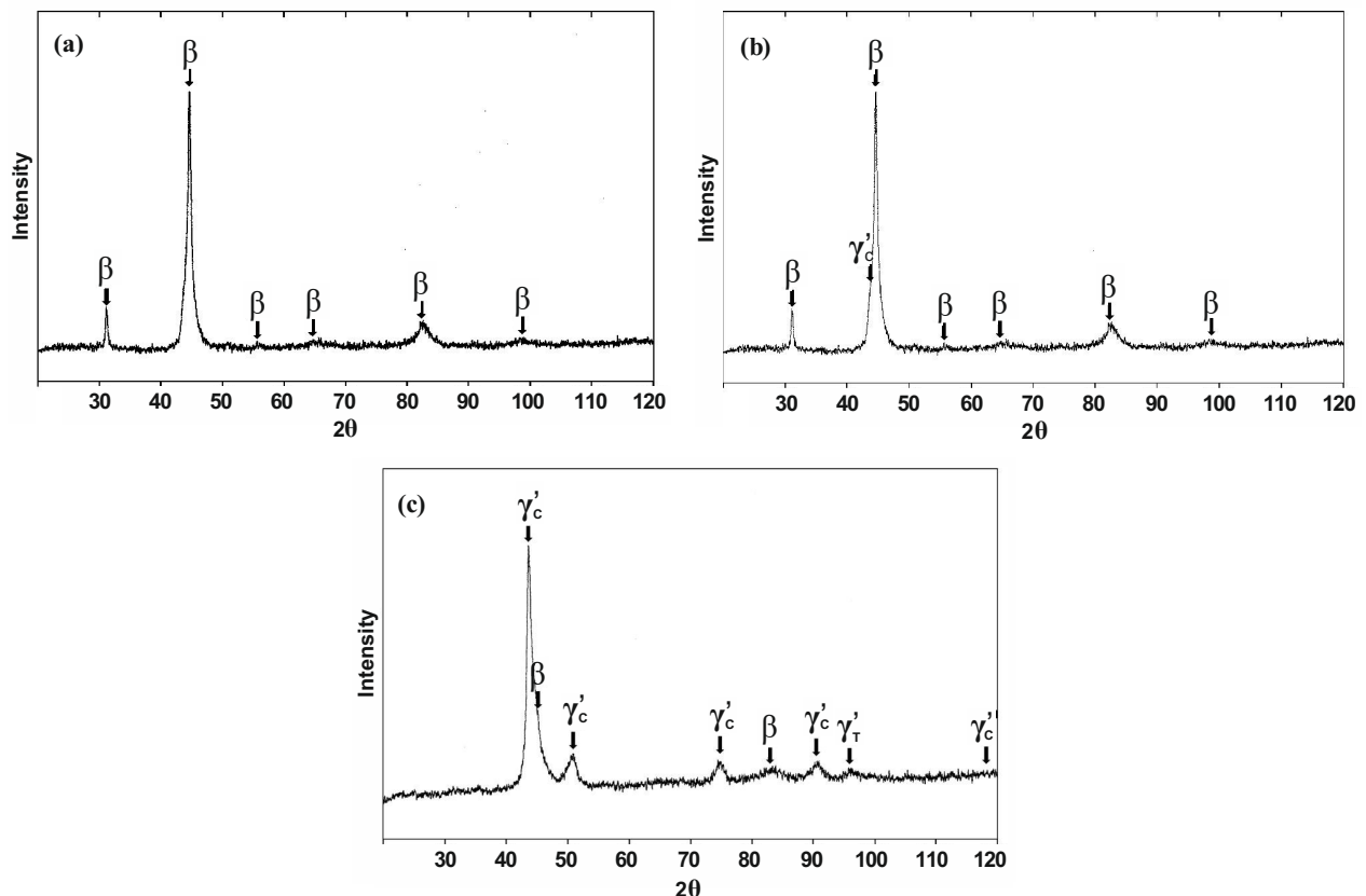
Fig. 1. X-ray diffraction of Cu–NiAl samples: NiAl 0.8 Cu 0.2 (a), NiAl 0.7 Cu 0.3 (b), and NiAl 0.6 Cu 0.4 (c).
