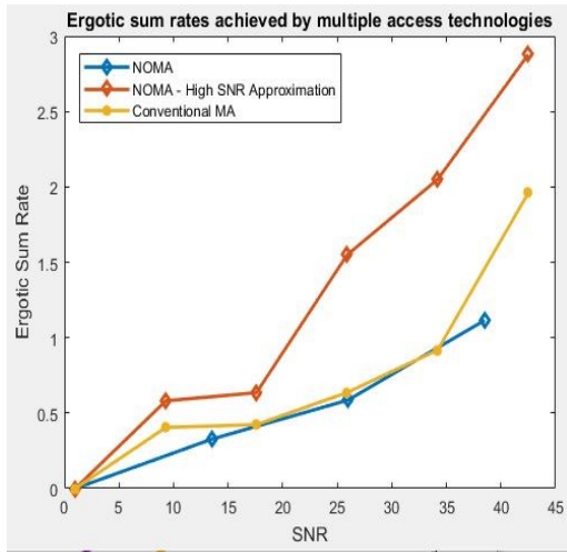
(a) Ergotic sum rates with high SNR value
