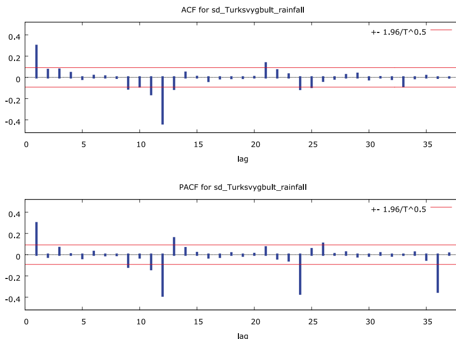
Fig. 3. Autocorrelation function (ACF) and partial autocorrelation function (PACF) plots of seasonally differenced rainfall time series; source; own study
