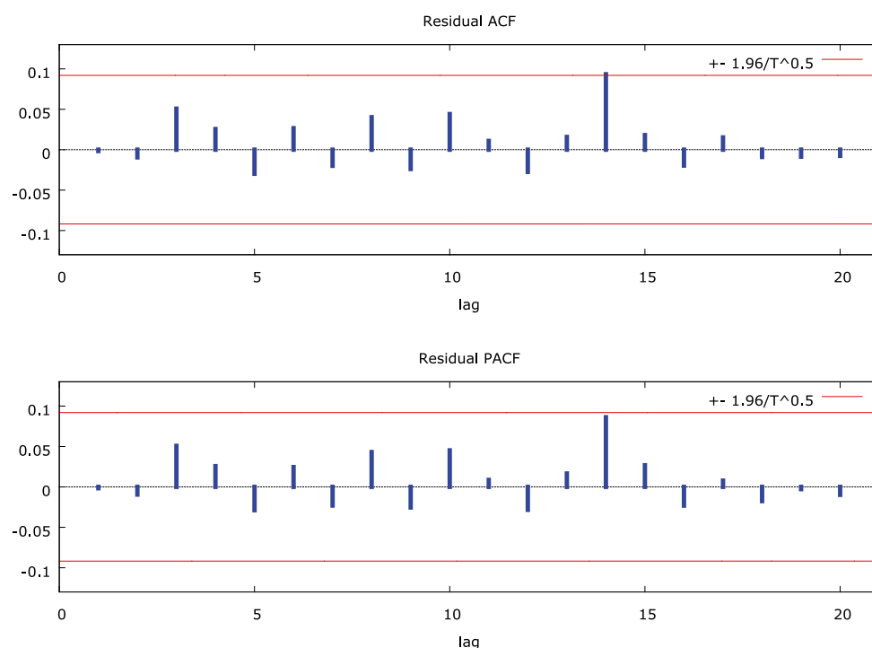
Fig. 6. Residual autocorrelation function (ACF) and partial autocorrelation functions (PACF) plots; source: own study
