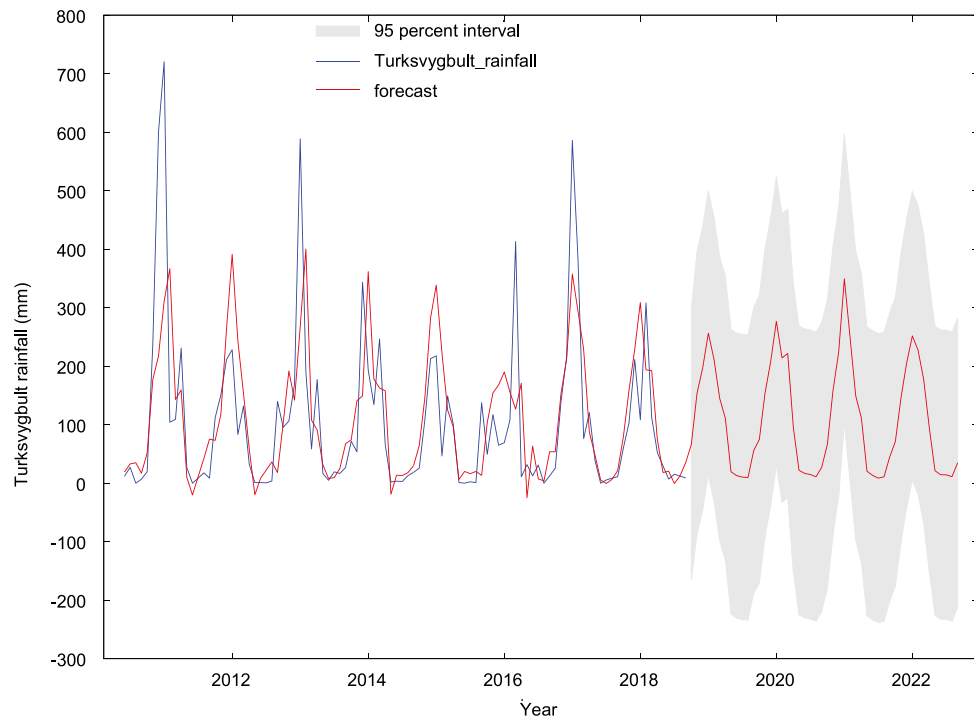
Fig. 4. SARIMA (2, 0, 3) (3, 1, 3) 12 model forecast of rainfall from 2019 to 2022 using GRETL software; source; own study
