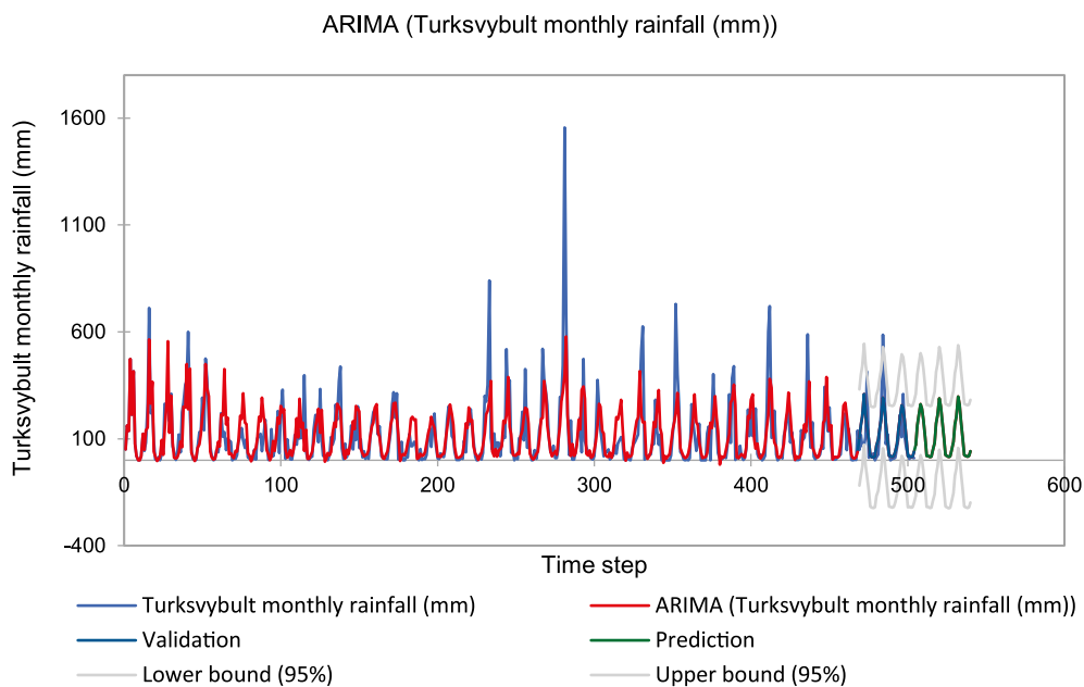
Fig. 5. SARIMA (1, 0, 1) (3, 1, 3) 12 forecast of rainfall using automatic XLSTAT software; source; own study
