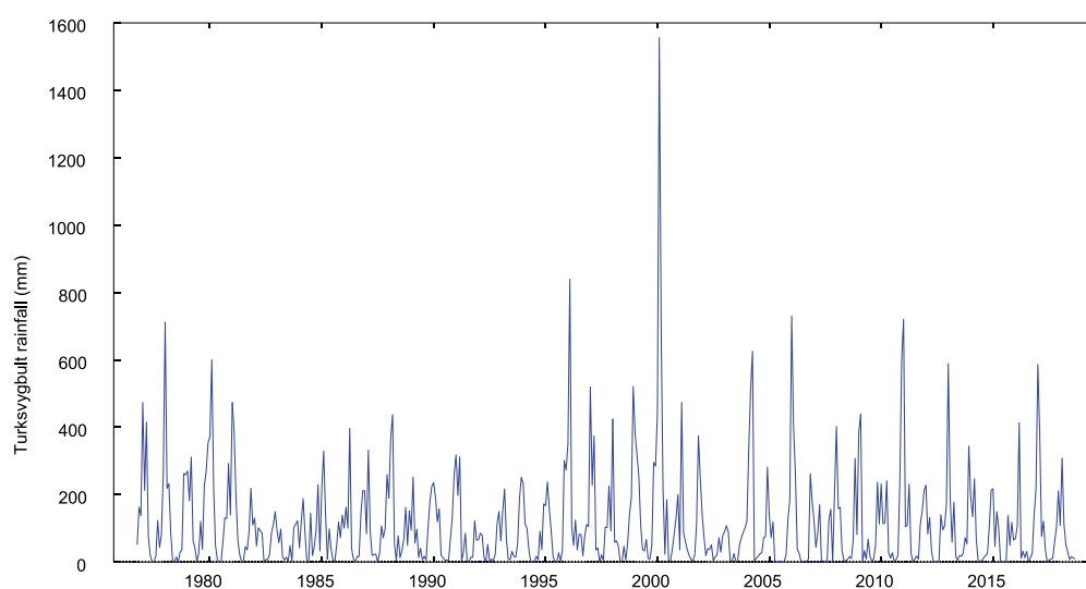
Fig. 1. Time series plot of the Turksvygbult rainfall from 1976 to 2018; source: own study
