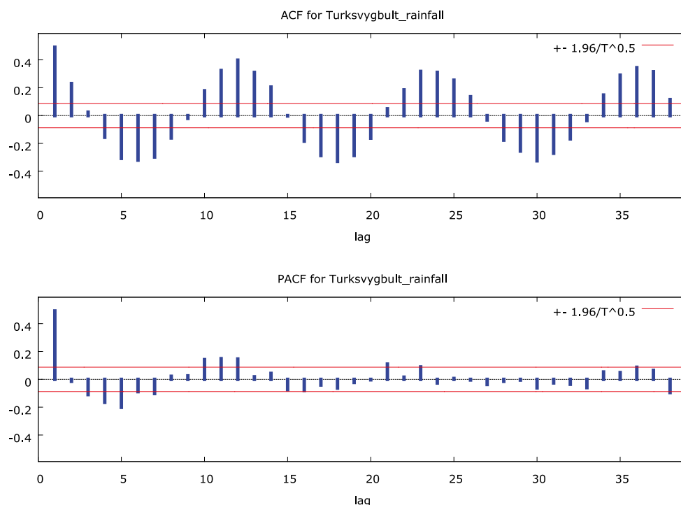
Fig. 2. Autocorrelation function (ACF) and partial autocorrelation function (PACF) plots of the rainfall time series for original data; source: own study
