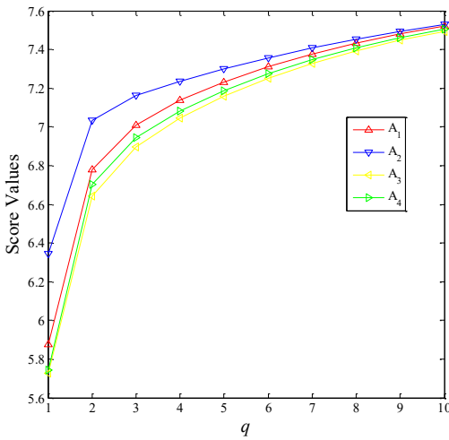
Figure 1: Score values of alternative for q \in [1, 10] based on L_q -ROFHPWA operator ( \zeta = 3 )
