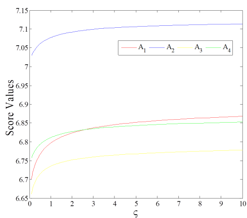
Figure 4: Score values of alternative for \varsigma \in (0, 10] based on Lq -ROFHPWG operator ( q = 3 )
