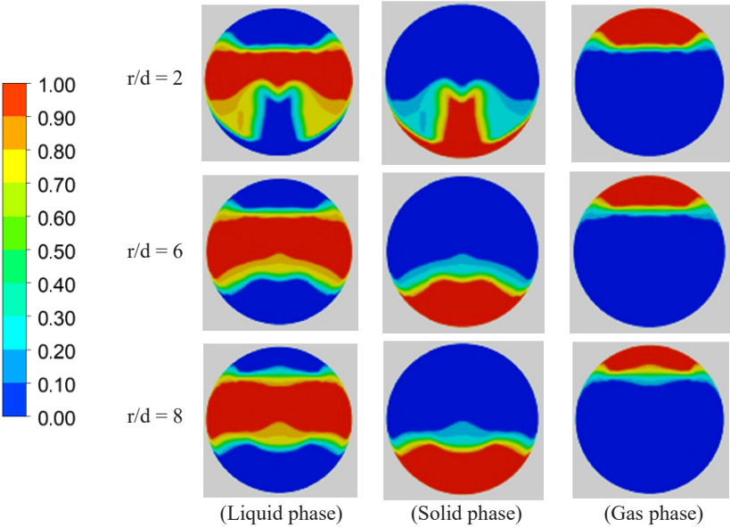
Fig. 12. At different bending diameter ratios, the volume fraction of each phase at the outlet (the speed is 4 m/s)
