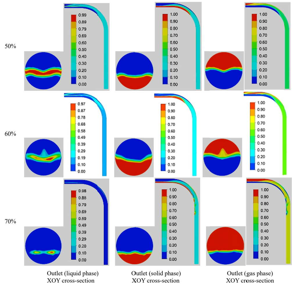
Fig. 15. XOY cross-section and volume score at exit when different gas volume fractions
