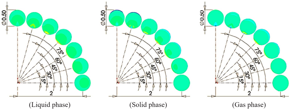
Fig. 9. Phase speed at each angle section of the bending segment
