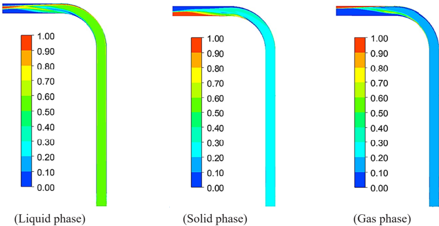
Fig. 4. Volume fraction on pipe XOY cross-section
