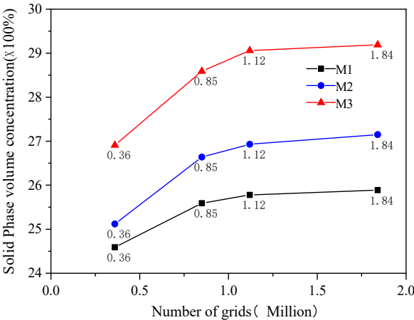
Fig. 3. Grid size-independent validation results
