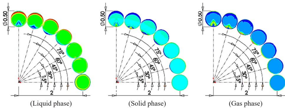
Fig. 6. Volume fractions of phases at each angle cross-section of the bending segment
