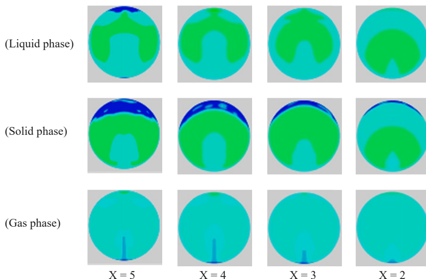
Fig. 10. Phase speed at each cross-section of the horizontal segment
