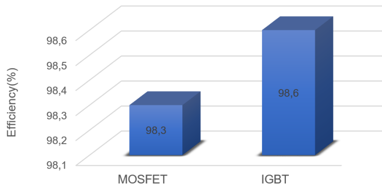
Fig. 12. Inverter efficiency
