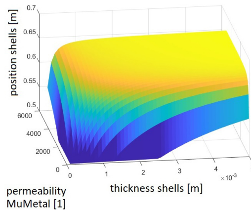
Fig. 8. A closer view of the singularity from Fig. 7
