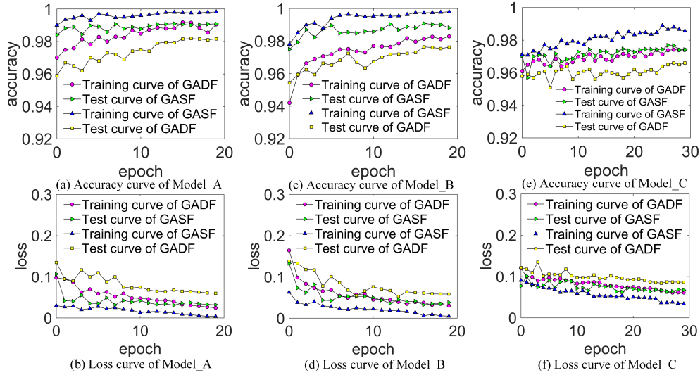
Fig. 6. Accuracy and loss value curve of sub-model under different inputs
