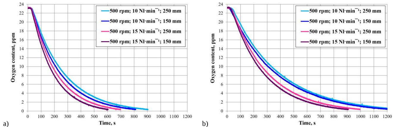
Fig. 5. Influence of the distance of the impeller above the bottom of the ladle on the concentration of oxygen for the impellers: (a) F2A 190, (b) J8 190 [10]
