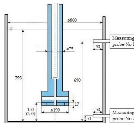
Fig. 2. Basic dimensional data of physical model [10]
