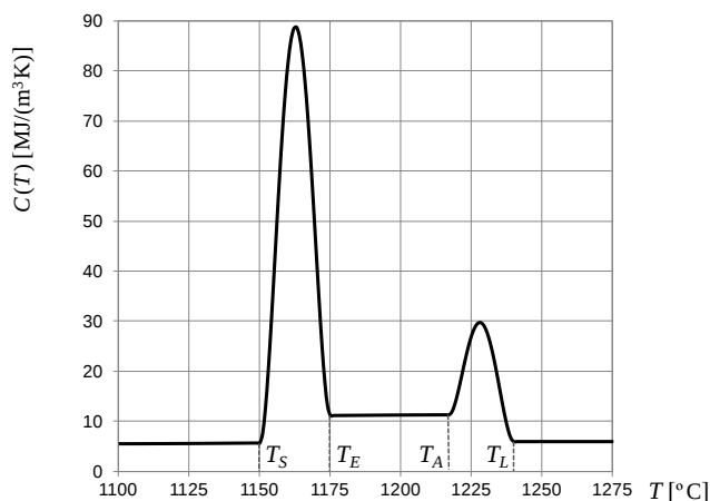
Fig. 3. Substitute thermal capacity of cast iron
