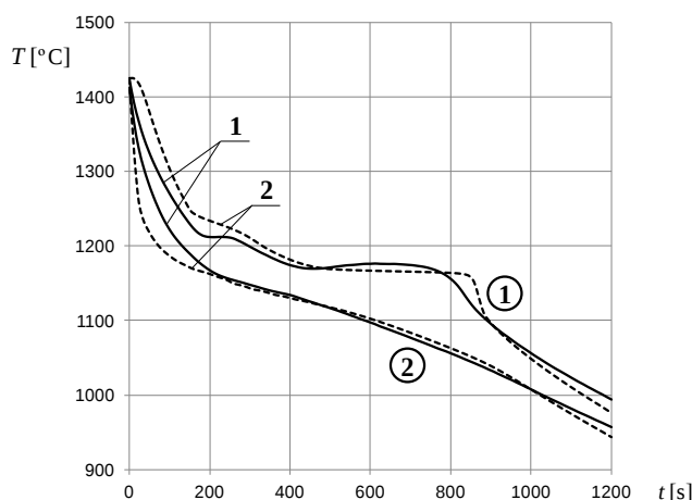
Fig. 5. Real (1) and calculated (2) cooling curves at points 1 and 2
