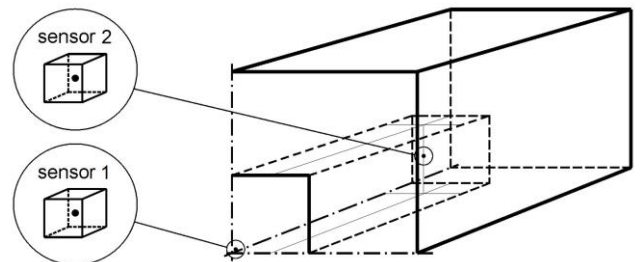
Fig. 2. Domain considered – casting of cuboid shape
