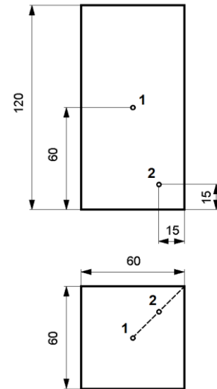
Fig. 1. Test casting – cuboid
