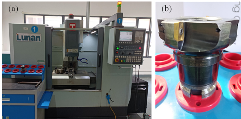
Fig. 6. (a) XHS7145 CNC machine. (b) TAP400R100-32-6T Disc Milling Cutter.
