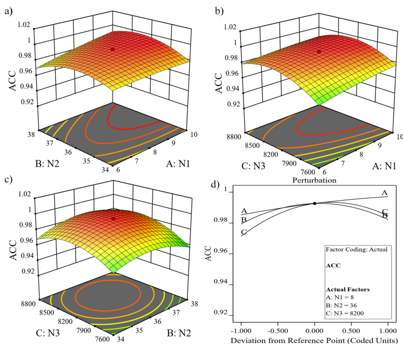
Fig. 10. 3D response surface diagram and perturbation diagram, ACC (accuracy).
