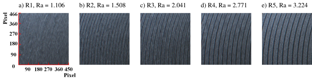
Fig. 9. Milling sample images for each roughness grade.
