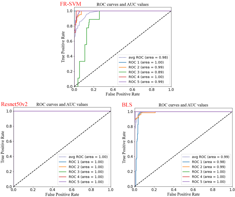
Fig. 12. ROC curves and AUC values for each model.
