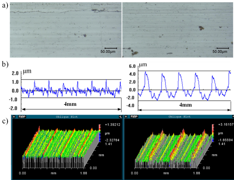
Fig. 1. Milling specimen (Left Ra 0.236 \mu\text{m} , Right Ra 1.477 \mu\text{m} ). a) Microscopic surface topography, b) roughness stylus measurement fluctuation graph, c) surface 3D morphology.
