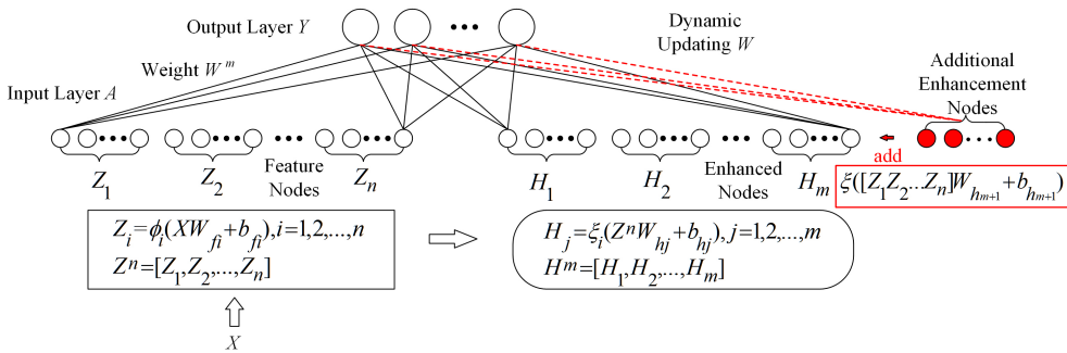
Fig. 2. Basic structure of broad learning system.
