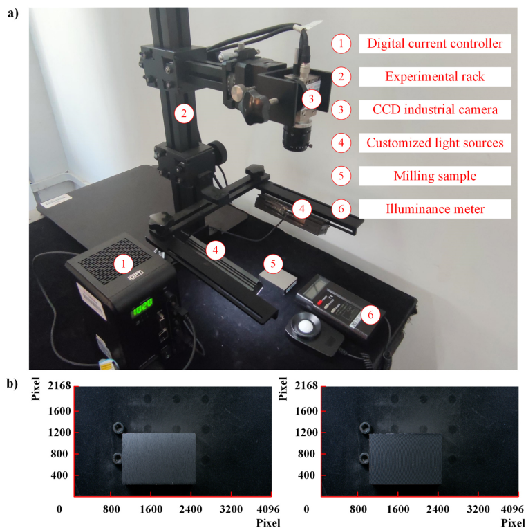
Fig. 7. a) Diagram of the experimental setup, b) milling workpiece image.
