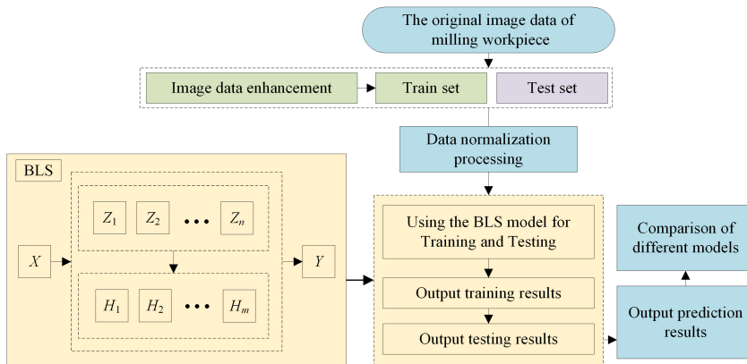
Fig. 4. Algorithm flow chart of the BLS roughness measurement model.
