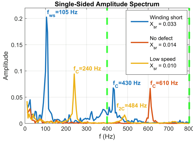
Fig. 14. The amplitude spectrum analysis where f_C are fundamental commutation frequencies, f_{2C} is the second harmonic of f_C and f_{ws} is a winding short fault. The area between dashed lines represents the required speed range (in this case 50-100%) for which the calculated X_{sr} thresholds are displayed. The X_{ws} threshold is defined as half of the f_C amplitude.
