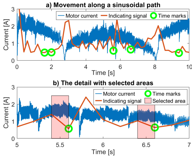
Fig. 13. Example of data selection based on the indicating signal.
