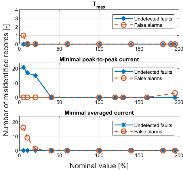
Fig. 11. Influence of input parameters on the jam detection method.
