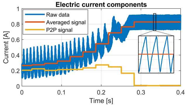
Fig. 8. Example of calculated components of electric current during the jam of an EMA.
