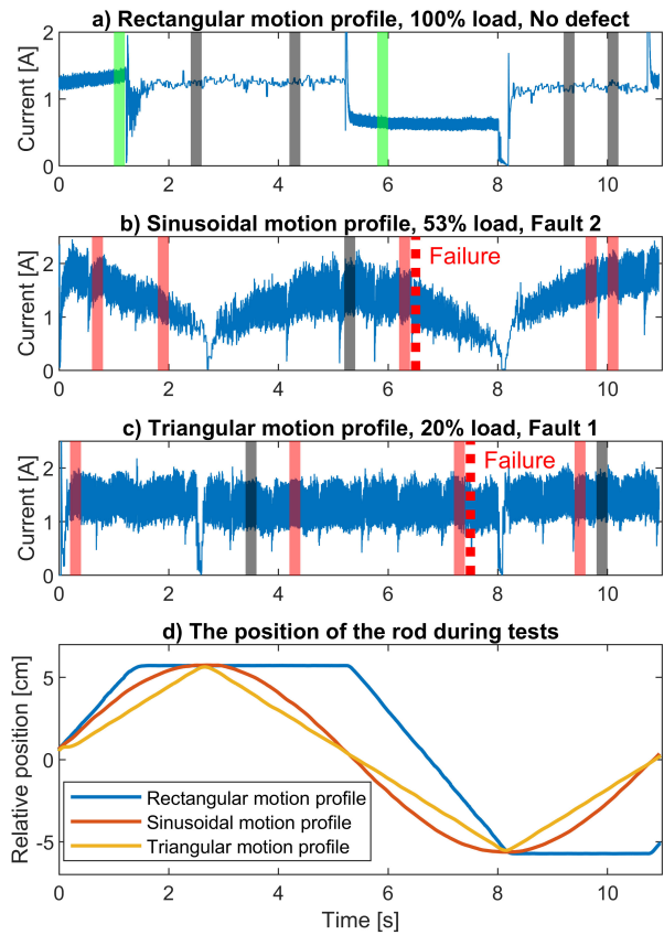
Fig. 15. Example of outcomes from the winding short detection algorithm (a, b, c) and the position of actuator rod recorded during these experiments (d). Highlighted stripes represent the data blocks selected for spectrum analysis, and their colour indicates results: green – no fault detected, red – a winding short detected, grey – data excluded from fault detection analysis (low or changing motor speed), a red dashed stripe – fault confirmed.
