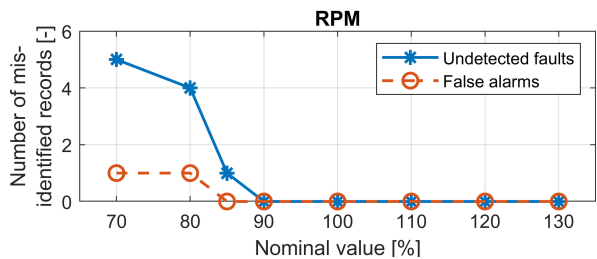
Fig. 17. Influence of input parameter on the winding short detection method.
