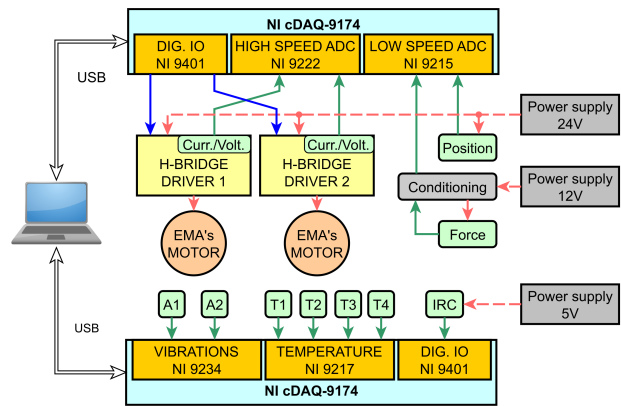
Fig. 5. Block diagram of the testing system.
