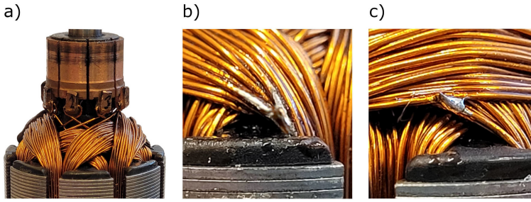
Fig. 12. Rotor winding – a) intact winding, b) detail of Fault 1, c) detail of Fault 2.
