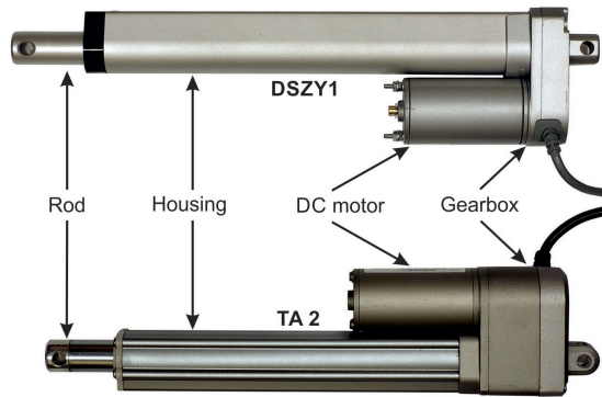
Fig. 6. DSZY1 and TA 2 actuators used during experiments.
