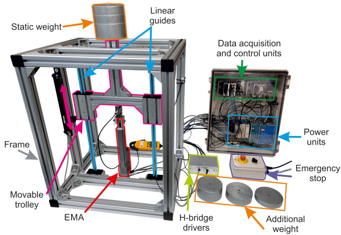
Fig. 7. Mechanical construction of the testing system with the TA 2 actuator.
