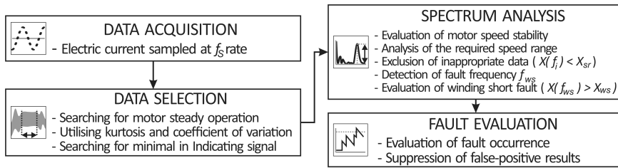
Fig. 3. Block diagram of the winding short detection algorithm.
