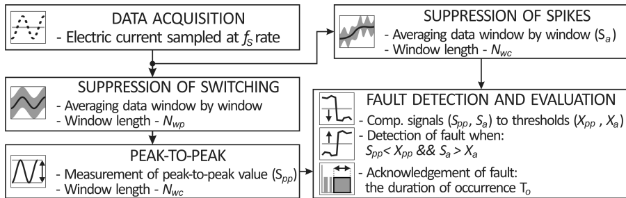
Fig. 2. Block diagram of the jam detection algorithm.
