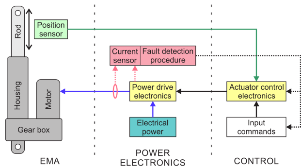
Fig. 4. Block diagram of the fault detection concept.
