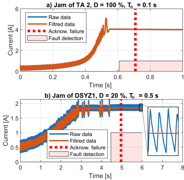
Fig. 9. Jam fault detection: a) hard stop, b) soft stop.
