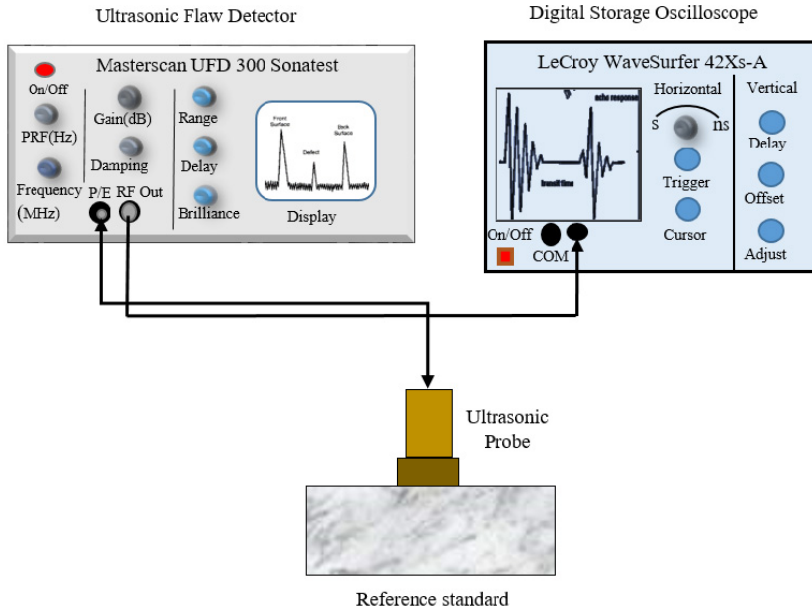
Fig. 3. Experimental setup for measurement of ultrasonic wave transit time in the RSB.
