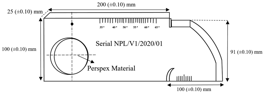
Fig. 1. Ultrasonic IIW V1 RSB (side view), used for the functional validation of UPE devices.
