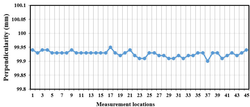
Fig. 7. Measured thickness variations for estimation of perpendicularity in the RSB.
