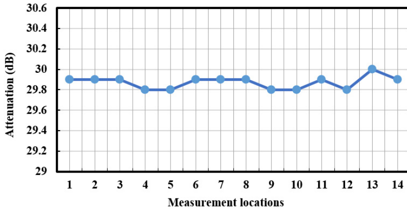
Fig. 5. Measured ultrasonic attenuation in the RSB.
