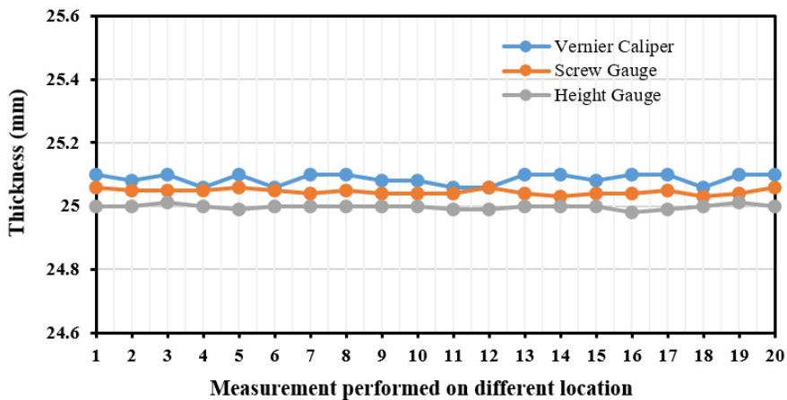
Fig. 2. Thickness measurement variation of the RSB by using the Vernier caliper, screw gauge, and height gauge.
