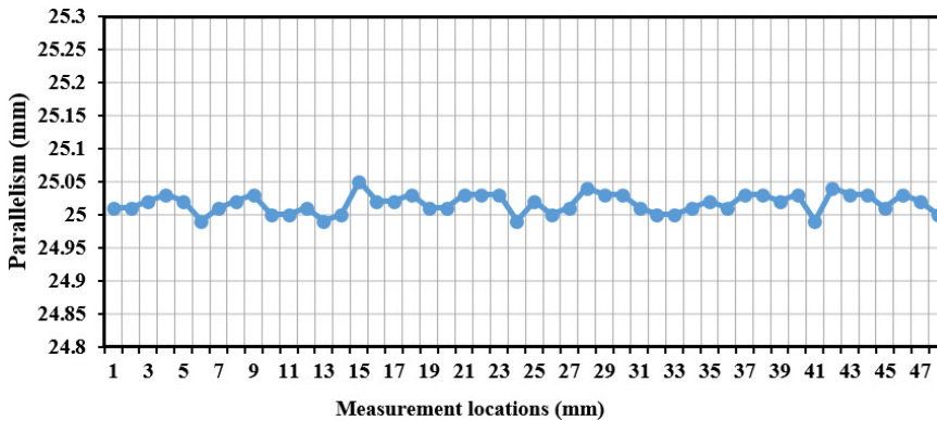
Fig. 6. Measured thickness variation for estimation of parallelism in the RSB.
