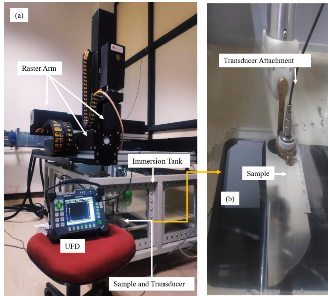
Fig. 4. a) Experimental setup for the immersion method, b) close view of the RSB and the transducer used in the immersion tank.
