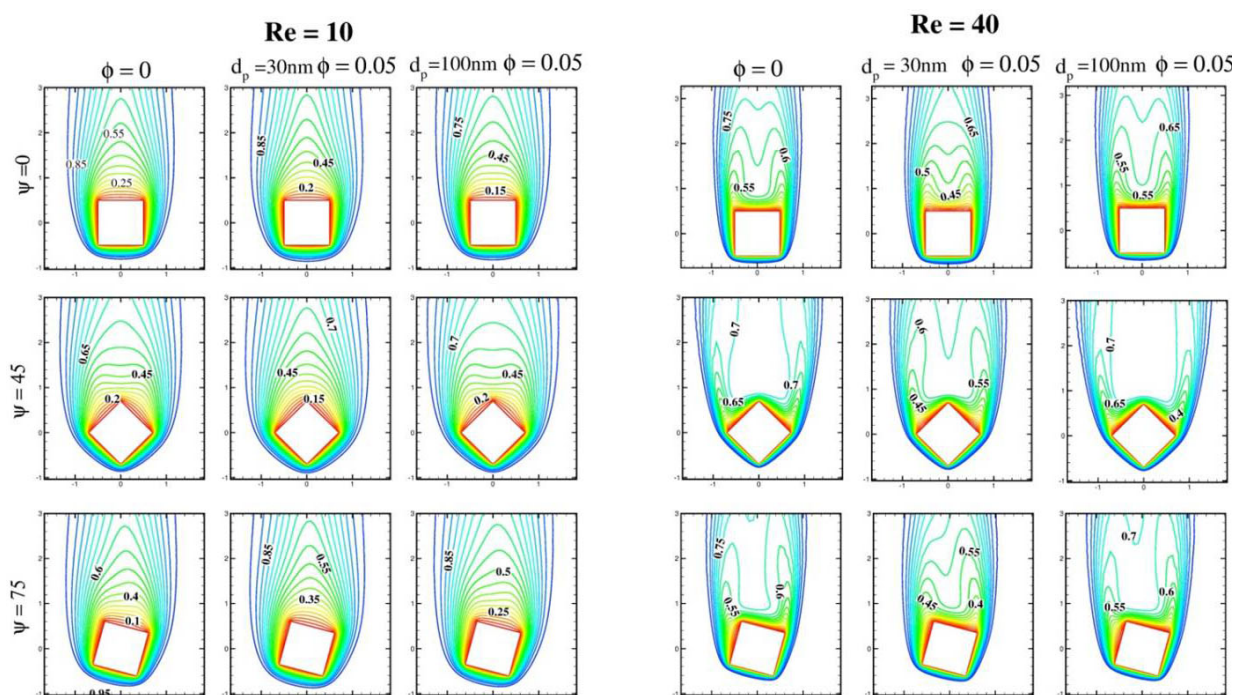
Fig. 2. Variation of isotherm contour with \text{Re} , d_{np} , \phi and orientation angle ( \psi )
