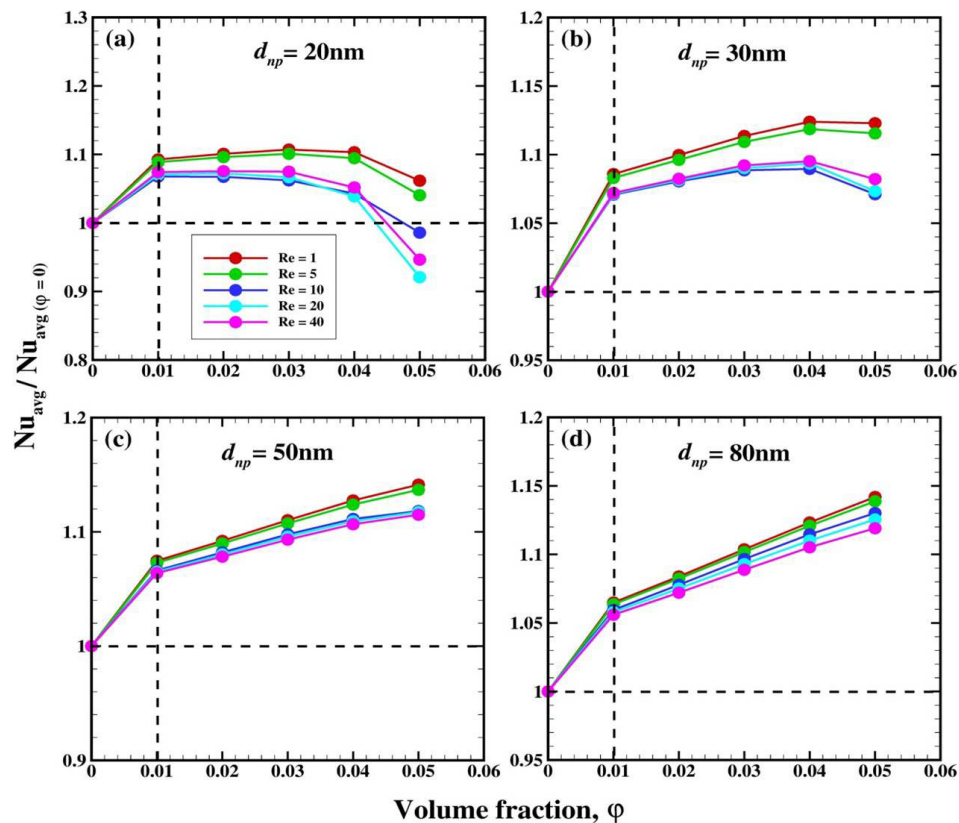
Fig. 4. Variation of E (for 45^\circ inclined square cylinder) with \phi of \text{CuO} \text{NPs}
