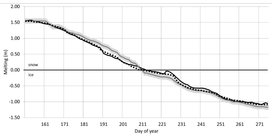
Fig. 3. The measured ablation on AWS2 (black line) with the ablation calculated from the temperature-index model (grey line) and energy balance model (dotted line). Bars indicate uncertainties.
