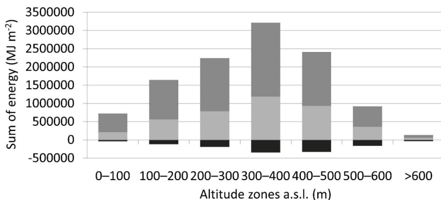
Fig. 6. Main components of the energy balance for altitude zones on Werenskioldbreen during the 2011 ablation season. Sensible heat is marked in light gray, the balance of shortwave radiation in dark gray and balance of longwave radiation in black.
