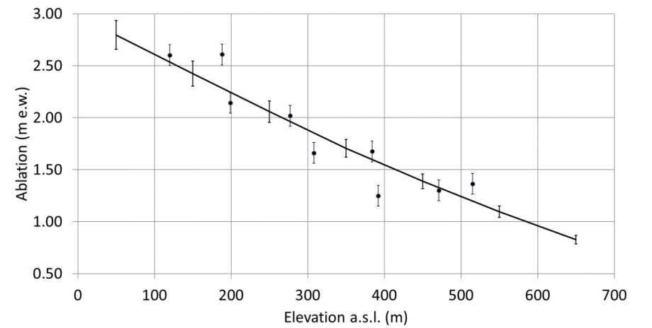
Fig. 4. The measured ablation on mass-balance stakes (black dots) with the ablation calculated from the temperature-index model (black line). Bars indicate uncertainties.
