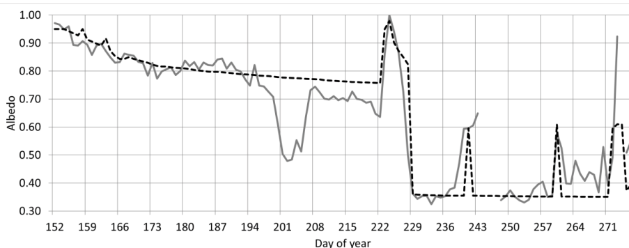
Fig. 5. Albedo measured on AWS2 (grey line) and modelled (dashed line) during the 2011 ablation season on Werenskioldbreen.
