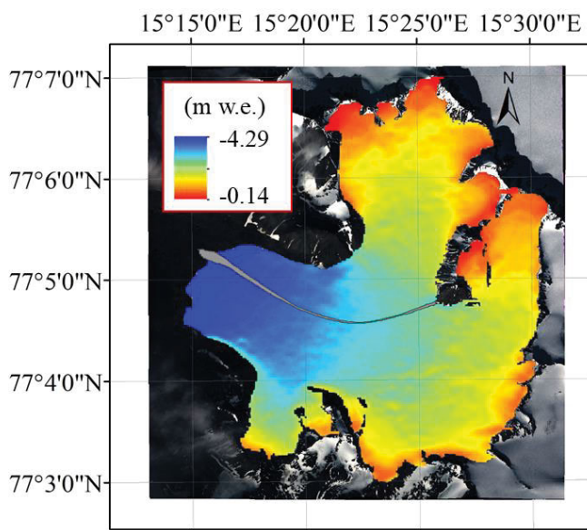
Fig. 8. Spatial distribution of ablation on Werenskioldbreen during the ablation season of 2011 on the basis of the energy balance model (background: GeoEye-1 VHSR image acquired on 10 August 2010).
