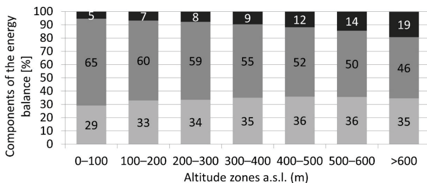
Fig. 7. Main components of the energy balance for altitude zones on Werenskioldbreen during the 2011 ablation season. Sensible heat is marked in light gray, the balance of shortwave radiation in dark gray and balance of longwave radiation in black.
