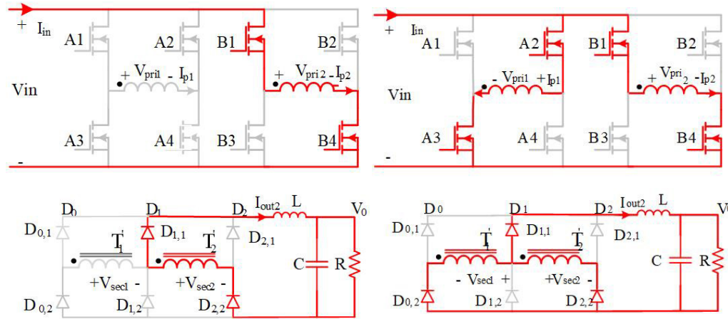
Fig. 6. Simplified diagram of mode D
