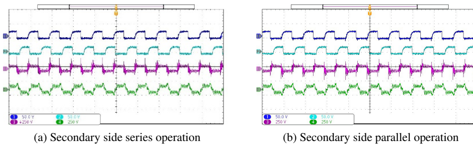
Fig. 14. The phase shift controls the secondary side series and parallel operation
