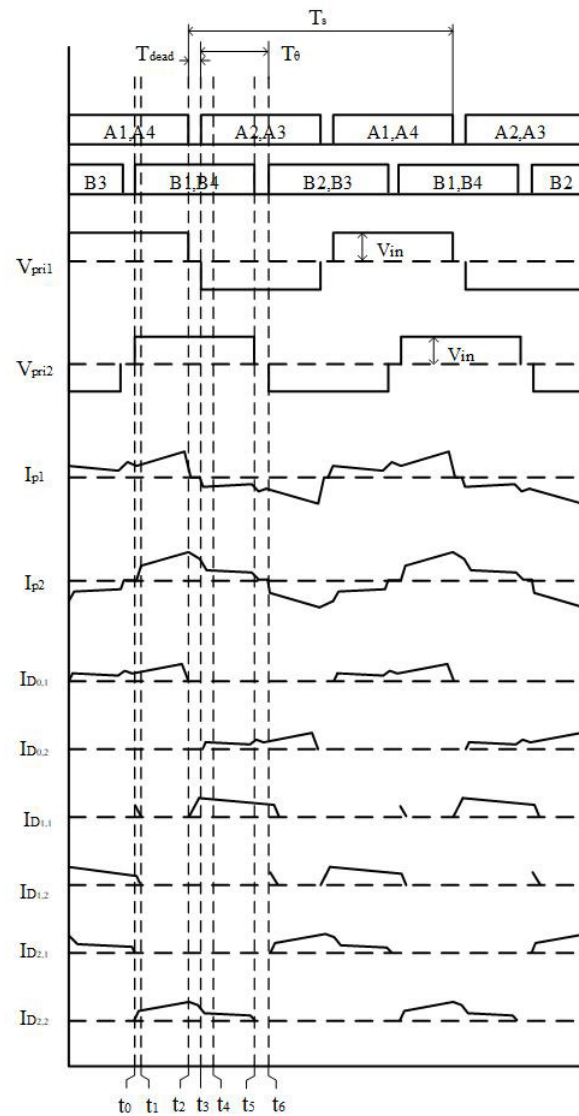
Fig. 8. Time series waveform
