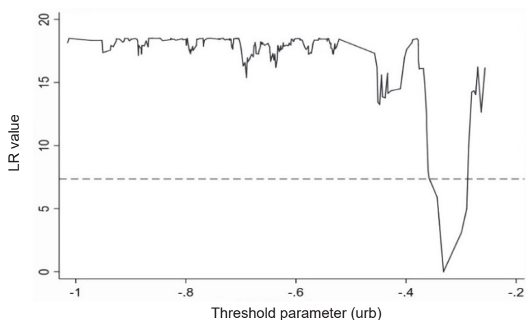
Fig. 2. Likelihood ratio function of the second threshold
