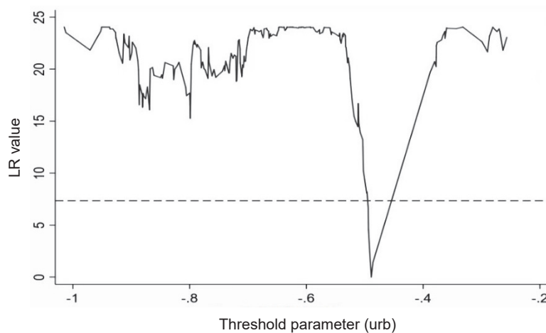
Fig. 1. Likelihood ratio function of the first threshold
