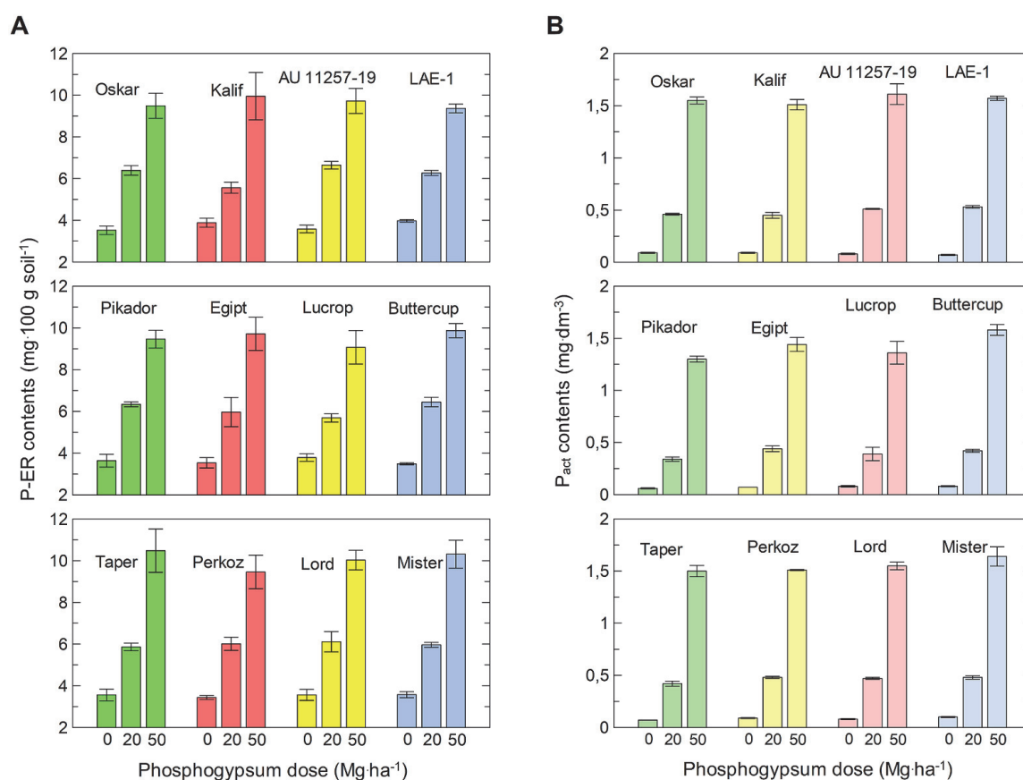
Fig. 2. (A) Content of available phosphorus determined by the Egner-Riehm method (P-ER) and (B) concentration of active phosphorus ( P_{\text{act}} ) in soil
