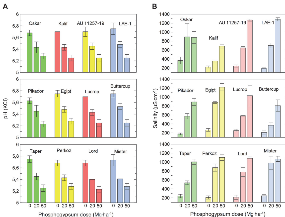
Fig 1. (A) Soil pH (KCl) and (B) soil salinity ( \mu\text{S}\cdot\text{cm}^{-1} )
