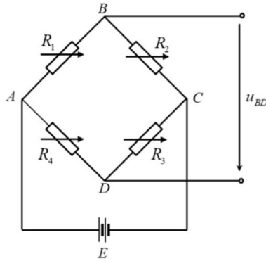
Fig. 5. Wheatstone bridge circuit for base strain measurement.
