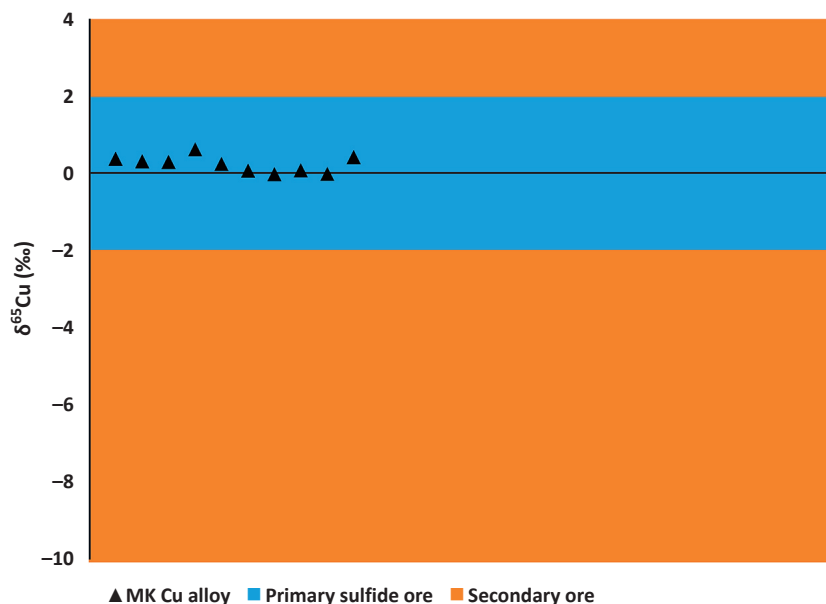
Results of the isotope analysis of copper from the copper objects found at Castillo de Huarmey compared against results for primary and secondary ores from copper mines from the Central Andes
