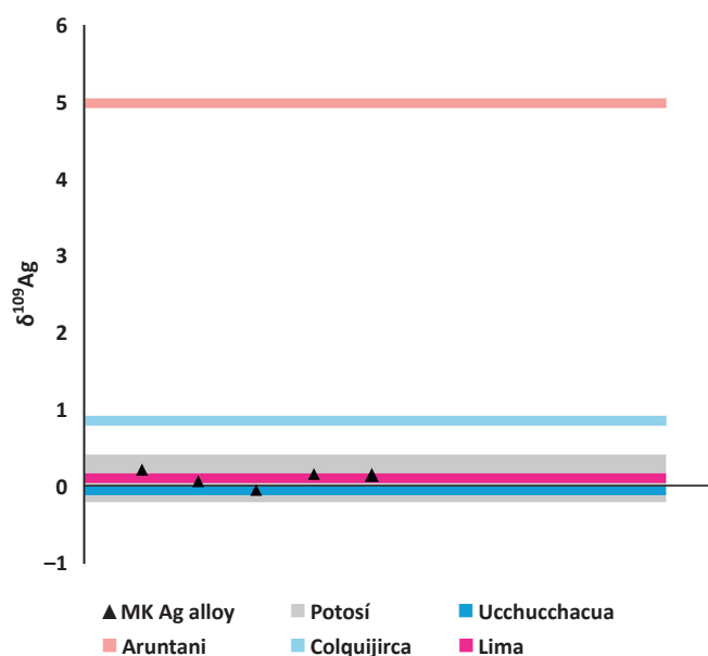
Results of the analysis of the isotopes of silver from the silver objects found at Castillo de Huarmey and analogous results from various silver mines from the Central Andes
