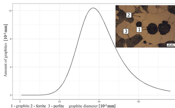
Fig. 2. Distribution of graphite particles amounts - melt II: U = 7.99 , W = 3.35 , Z = 2.58
