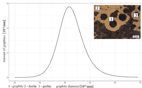
Fig. 3. Distribution of graphite particles amounts - melt V: U = 7.99 , W = 3.61 , Z = 6.21
