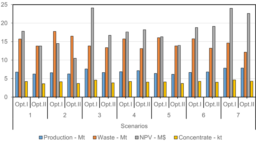
Fig. 5. Chart of comparison of optimization results
