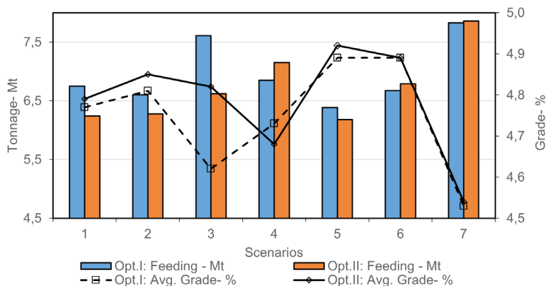
Fig. 7. Comparison of plant feed tonnage and mean grades produced by optimizations
