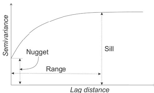
Fig. 1. Important characteristics of a semivariogram (own elaboration)
