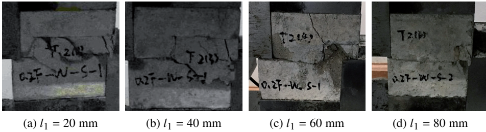
Fig. 9. Post-shear-test damage morphology in specimens with a single-ladder step joint under normal stress of 3.03 MPa, given h = 20 mm and variable l_1
