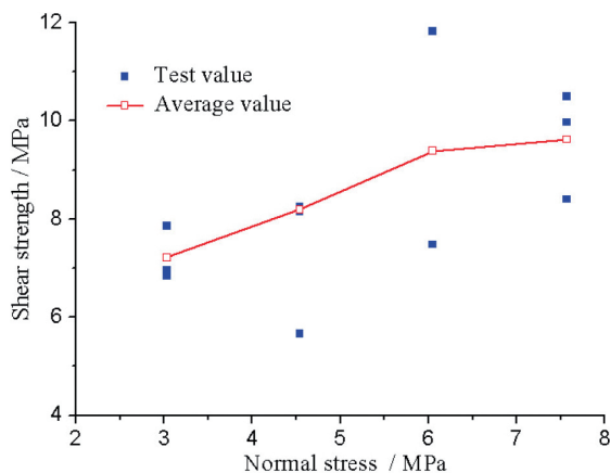
Fig. 4. Shear strengths of intact specimens
