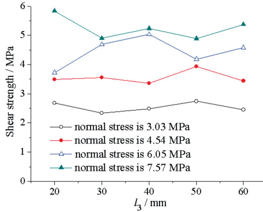
Fig. 13. Variation of shear strength with l_3 in specimens with a single-rectangular step joint, given l_5 = 20 mm and h = 20 mm
