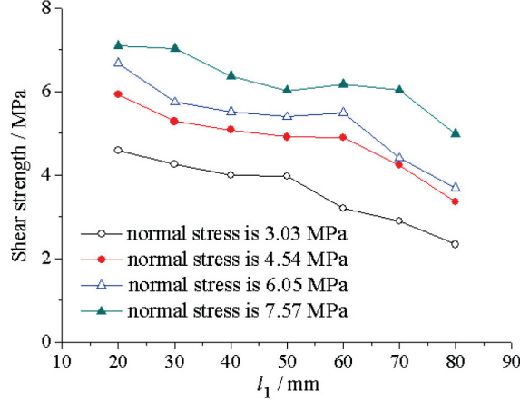
Fig. 6. Shear strengths of specimens with a single-ladder step joint with fixed h = 20 mm and variable l_1
