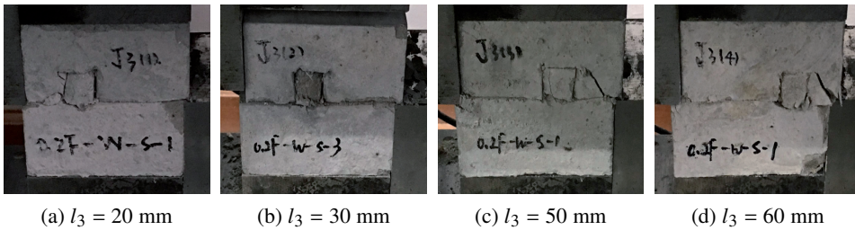
Fig. 18. Post-shear-test damage morphology in specimens with a single-rectangular step joint, given l_5 = 20 mm and normal stress of 3.03 MPa
