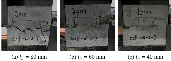
Fig. 17. Post-shear-test damage morphology in specimens with a single-ladder step joint, given fixed l_3 = l_4 , h = 20 mm and normal stress of 7.57 MPa
