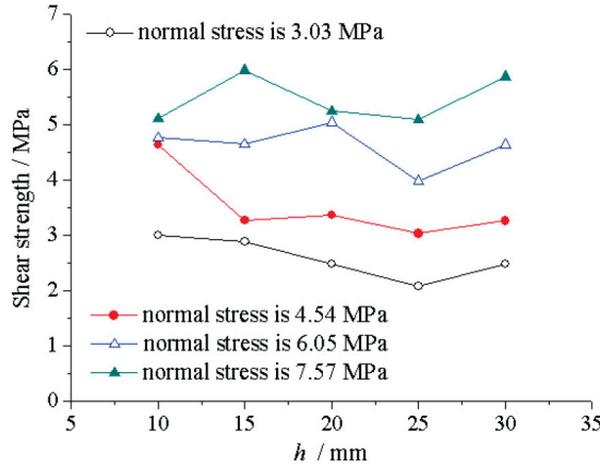
Fig. 11. Variation of shear strength with h in specimens with a single-rectangular step joint, given l_3 = l_4 = 40 mm and l_5 = 20 mm
