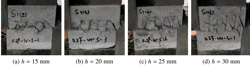
Fig. 21. Post-shear-test damage morphology in specimens with a single-ladder step joint, given fixed l_3 = l_4 = 50 mm and normal stress of 3.03 MPa
