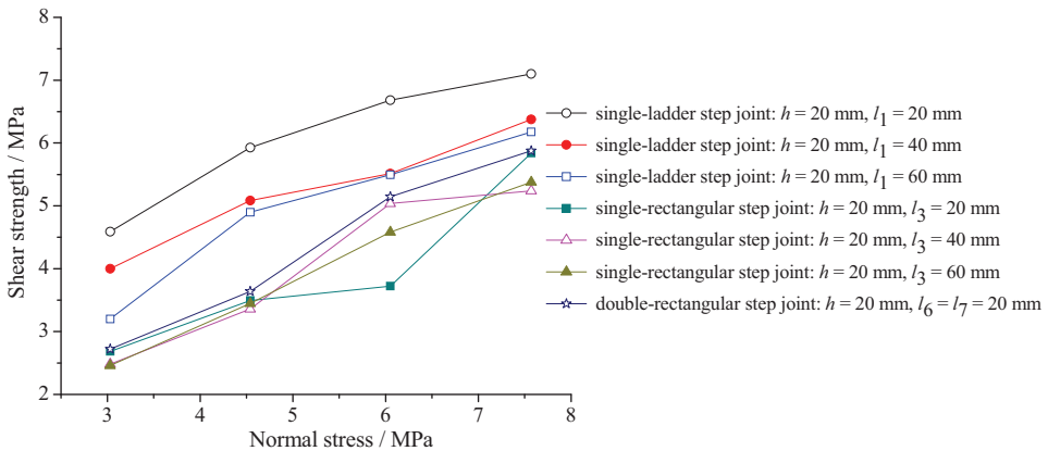
Fig. 22. Comparison results of the shear strength in specimens with three kinds of step joint
