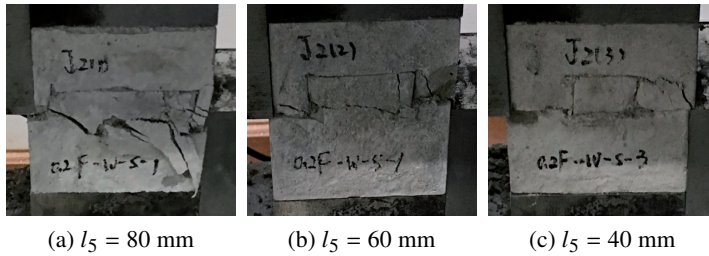
Fig. 16. Post-shear-test damage morphology in specimens with a single-ladder step joint, given fixed l_3 = l_4 , h = 20 mm and normal stress of 3.03 MPa
