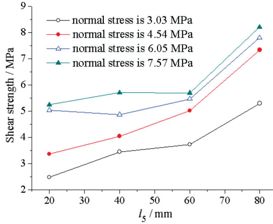
Fig. 12. Variation of shear strength with l_5 in specimens with a single-rectangular step joint, given l_3 = l_4 and h = 20 mm
