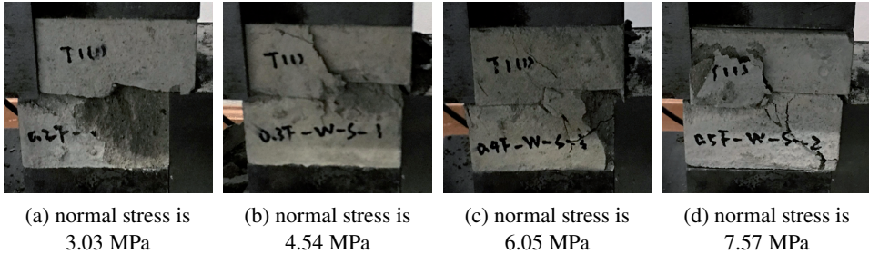
Fig. 7. Post-shear-test damage morphology in specimens with a single-ladder step joint, given fixed l_1 = l_2 = 50 mm and h = 10 mm
