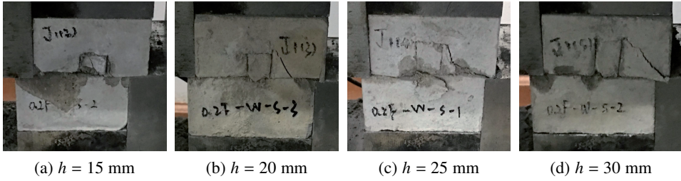
Fig. 15. Post-shear-test damage morphology in specimens with a single-ladder step joint, given fixed l_3 = l_4 = 50 mm and normal stress of 3.03 MPa
