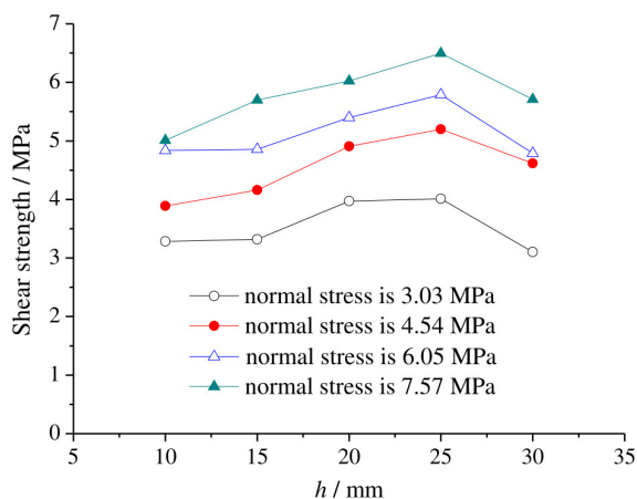
Fig. 5. Shear strengths of specimens with a single-ladder step joint with fixed l_1 = l_2 = 50 mm and variable h
