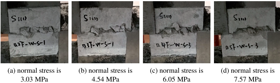
Fig. 20. Post-shear-test damage morphology in specimens with a single-rectangular step joint, given fixed l_3 = l_4 = 50 mm and h = 10 mm
