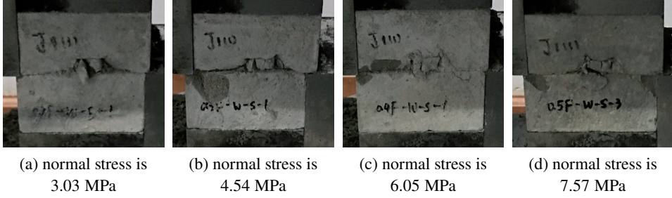
Fig. 14. Post-shear-test damage morphology in specimens with a single-rectangular step joint, given fixed l_3 = l_4 = 50 mm and h = 10 mm
