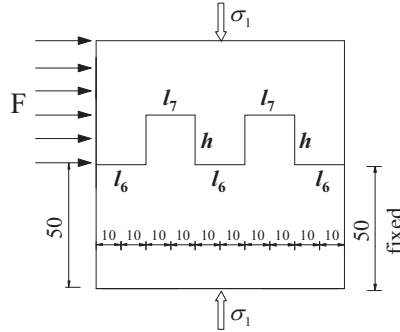
Fig. 3. Shear test diagram for specimens with a double-rectangular step joint (unit: mm)
