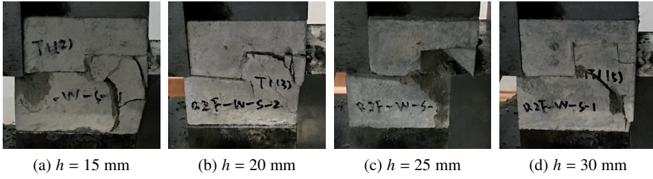
Fig. 8. Post-shear-test damage morphology in specimens with a single-ladder step joint, given fixed l_1 = l_2 = 50 mm and normal stress of 3.03 MPa
