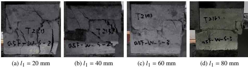
Fig. 10. Post-shear-test damage morphology in specimens with a single-ladder step joint under normal stress of 7.57 MPa, given fixed h = 20 mm and variable l_1
