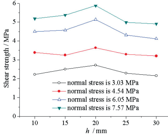
Fig. 19. Variation of shear strength of specimens with h with a double-rectangular step joint, given l_6 = l_7 = 20 mm
