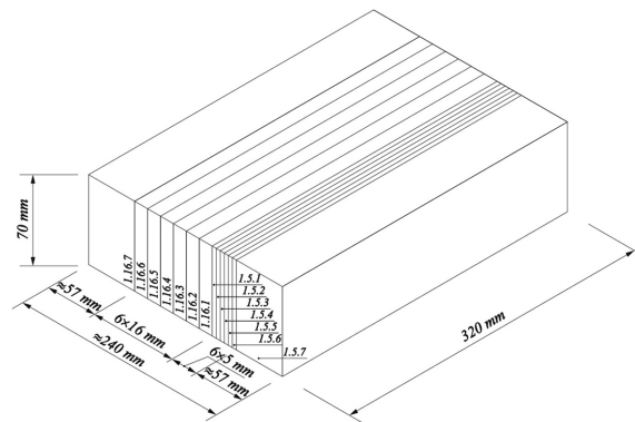
Fig. 1. The hot rolled steel plate (70 × 240 × 320 mm)
