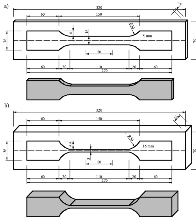
Fig. 2. The flat samples: a) 5 mm, b) 16 mm
