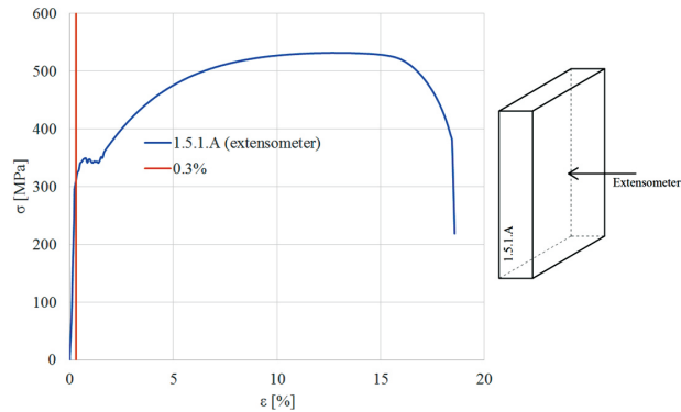
Fig. 7. Stress-strain curves for sample 1.5.1.A
