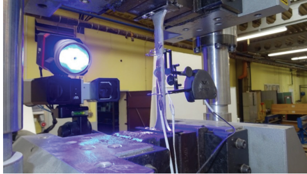
Fig. 3. Variant B of instruments configuration (5 mm sample)
