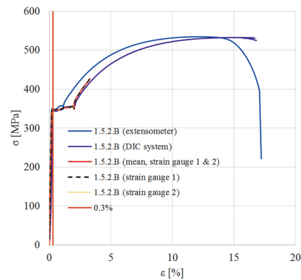
Fig. 8. Stress-strain curves for sample 1.5.2.B
