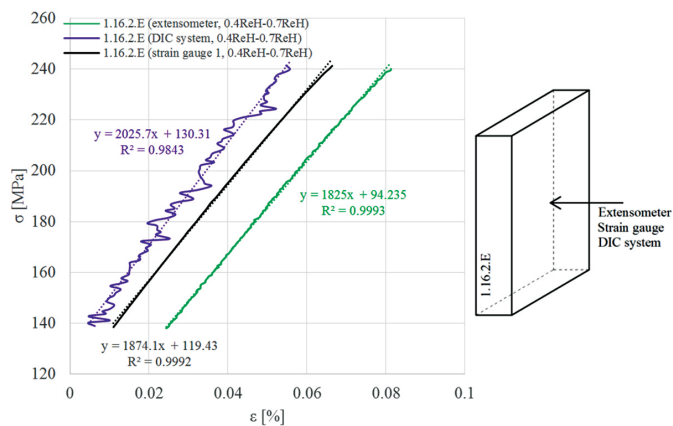
Fig. 15. The straight lines determined between 40% of R_{eH} and 70% of R_{eH} with the coefficient of determination R^2 for sample 1.16.2.E, and the instrument configuration
