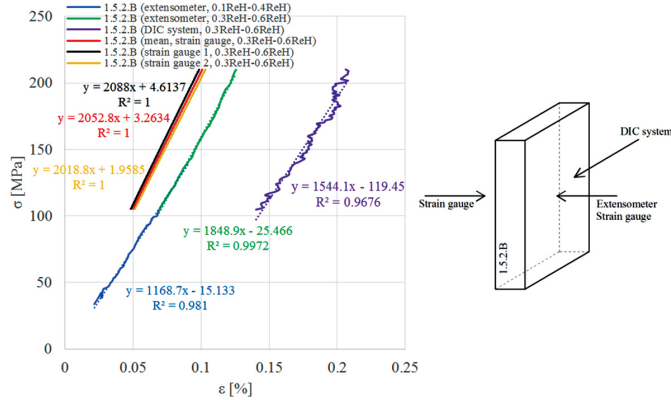
Fig. 9. The straight lines determined between 10% of R_{eH} and 40% of R_{eH} , and between 30% of R_{eH} and 60% of R_{eH} with the coefficient of determination R^2 for sample 1.5.2.B, and the instrument configuration
