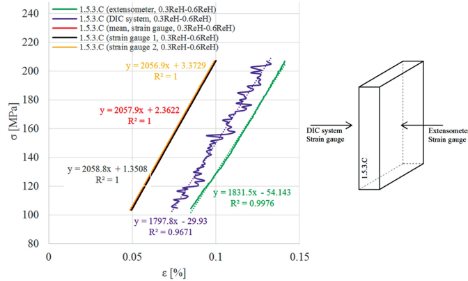
Fig. 11. The straight lines determined between between 30% of R_{eH} and 60% of R_{eH} with the coefficient of determination R^2 for sample 1.5.3.C, and the instrument configuration
