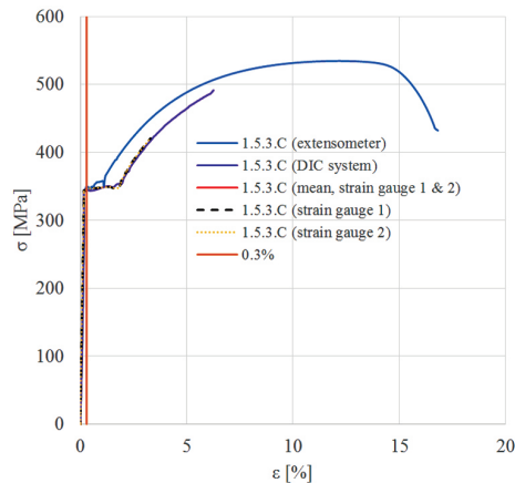
Fig. 10. Stress-strain curves for sample 1.5.3.C
