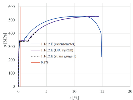
Fig. 14. Stress-strain curves for sample 1.16.2.E
