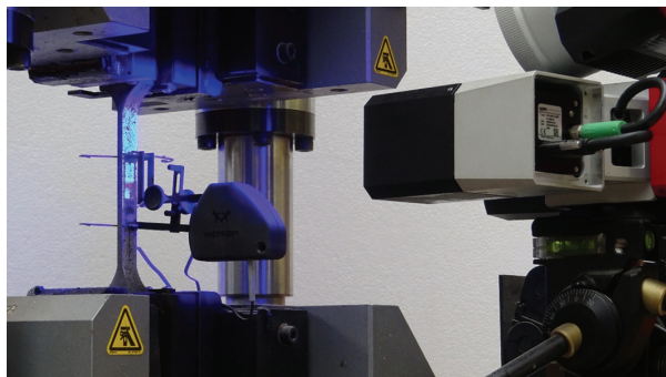
Fig. 5. Variant E of instruments configuration (16 mm sample)
