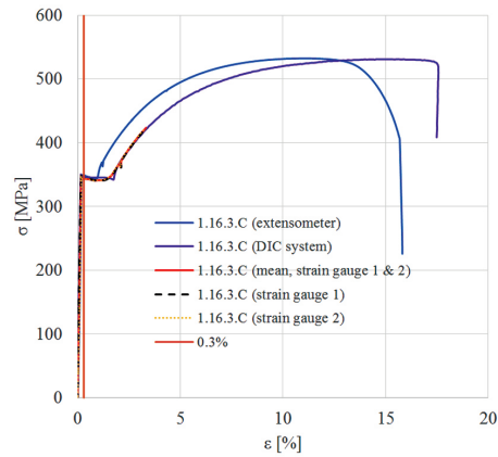
Fig. 16. Stress-strain curves for sample 1.16.3.C
