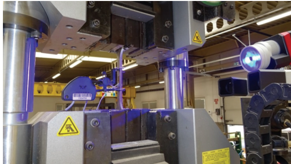
Fig. 4. Variant C of instruments configuration (5 mm sample)
