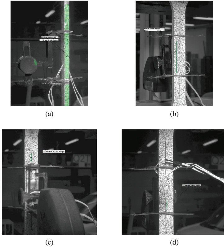
Fig. 6. Virtual strain gauges used for: a) 1.5.2.B specimen, b) 1.5.3.C specimen, c) 1.16.2.E specimen, d) 1.16.3.C specimen
