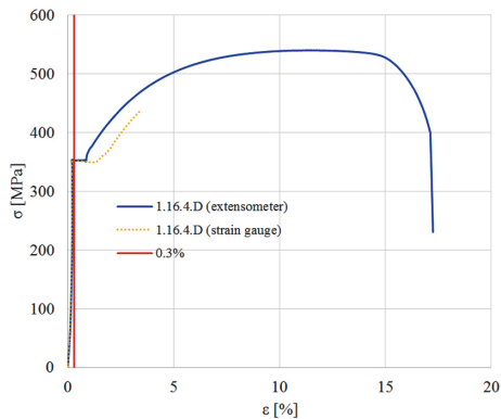
Fig. 18. Stress-strain curves for sample 1.16.4.D
