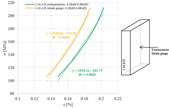
Fig. 19. The straight lines determined between 30% of R_{eH} and 60% of R_{eH} with the coefficient of determination R^2 for sample 1.16.4.D, and the instrument configuration
