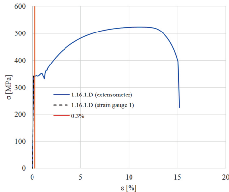
Fig. 12. Stress-strain curves for sample 1.16.1.D
