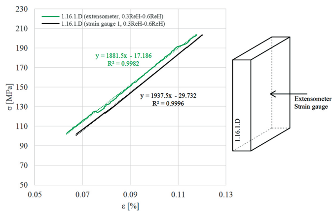
Fig. 13. The straight lines determined between 30% of R_{eH} and 60% of R_{eH} with the coefficient of determination R^2 for sample 1.16.1.D, and the instrument configuration
