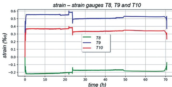
Fig. 9. Example strain plot vs. time for selected strain gauges
