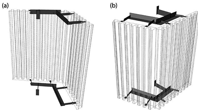
Fig. 11. Rear (a) and front (b) views of the finite-element model
