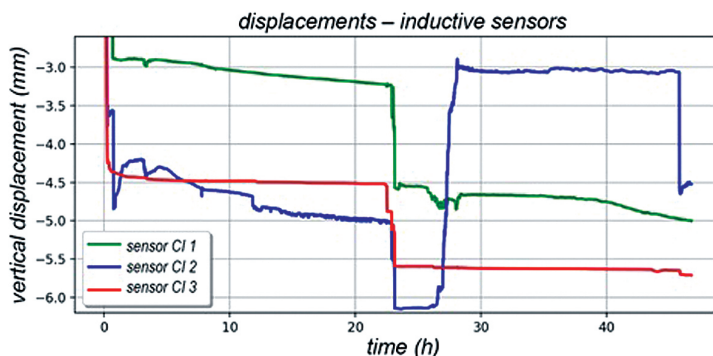
Fig. 8. Example displacement-time graph for the selected inductive sensors
