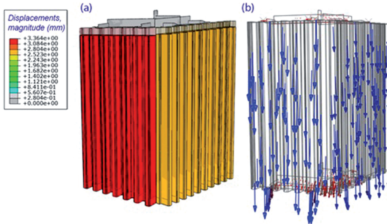
Fig. 12. Displacements: (a) contour map (b) vector map of displacements
