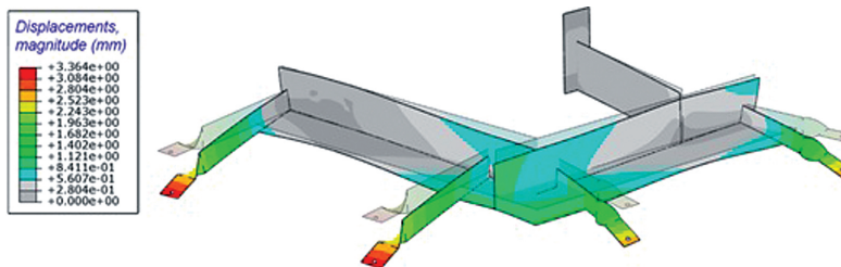
Fig. 13. Resultant displacements of the lower framework – unstrained and strained (scaled 20 times)
