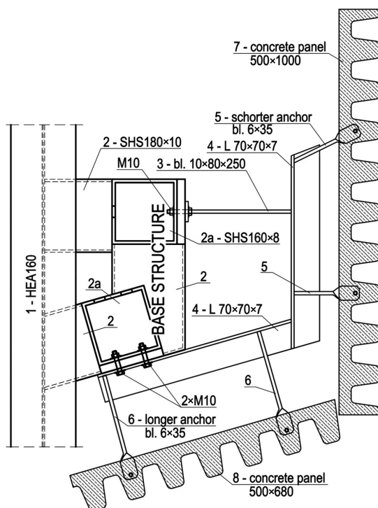
Fig. 2. Schematic representation of the tested mock-up
