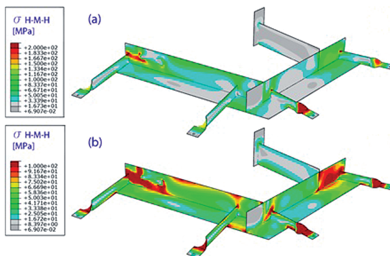
Fig. 14. Contour maps of von Mises equivalent stresses. Two different colour scales were applied
