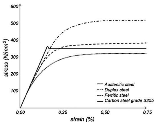
Fig. 6. Stress-strain curves of stainless and carbon steels
