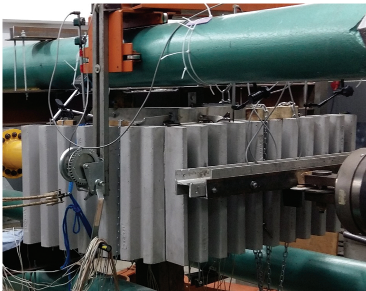
Fig. 3. Overview of the curtain wall mock-up installed in the test stand
