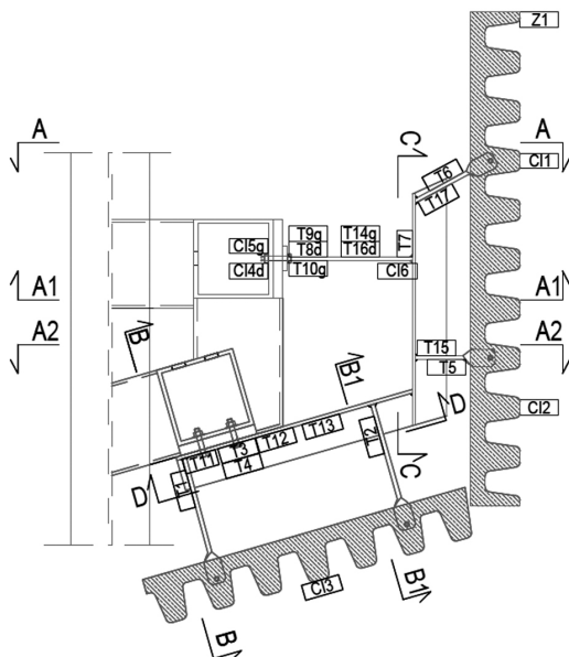
Fig. 4. Placement of inductive sensors (CI) and strain gauges (T) – top view
