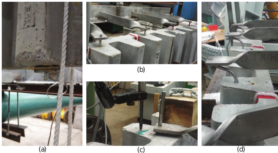
Fig. 7. Failure modes of the curtain wall components: fracture of mortar where the panel rests on the anchor (a), steel bolts forced out of the concrete panels (b), bolt forced out of the flat bar anchor (c), bolts forced out and bent thereafter (d)
