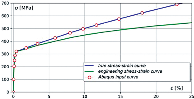
Fig. 10. Averaged stress-strain curves for steel grade 1.4301
