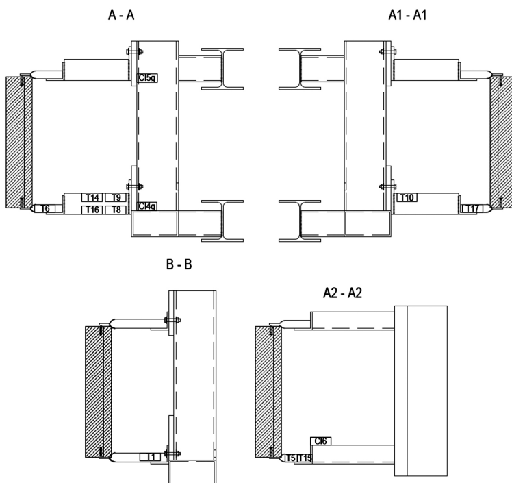
Fig. 5. Placement of inductive sensors (CI) and strain gauges (T) – cross-sections
