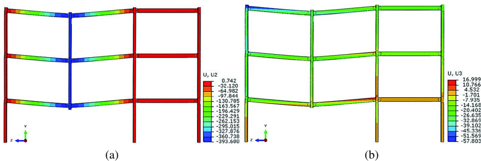
Fig. 13. View of frame under sudden column loss at final stage of analysis: a) vertical displacement, b) horizontal displacement
