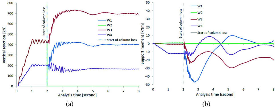
Fig. 10. Response curves of three bays frame with 15 mm thickness extended end-plate joint under sudden column loss: a) vertical reaction – time analysis, b) support moment vs. time analysis
