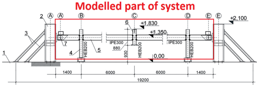
Fig. 2. Planar view of frame substructure tested in [12, 19]
