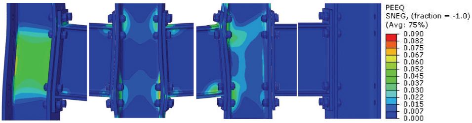
Fig. 14. Map of strains of joint (from left W5 to W8) with 15 mm thickness extended end-plate at level of structure +3.50 at final stage of analysis
