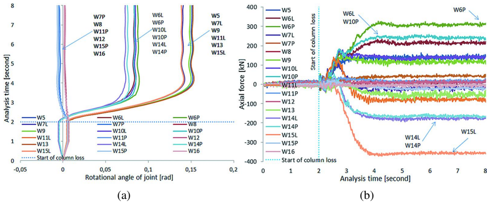
Fig. 12. Curves of: a) time analysis – rotational angle of joints, b) axial force – time analysis
