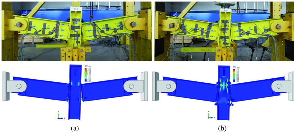
Fig. 1. Comparison views of experimental test [13] and numerical analysis [16] of joint: a) 10 mm flush end-plate, b) 10 mm extended end-plate
