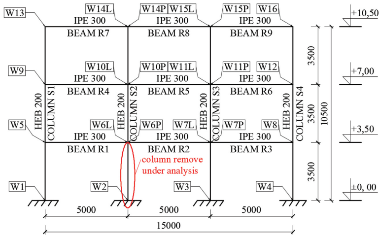
Fig. 9. Static diagram of the analyzed frame
