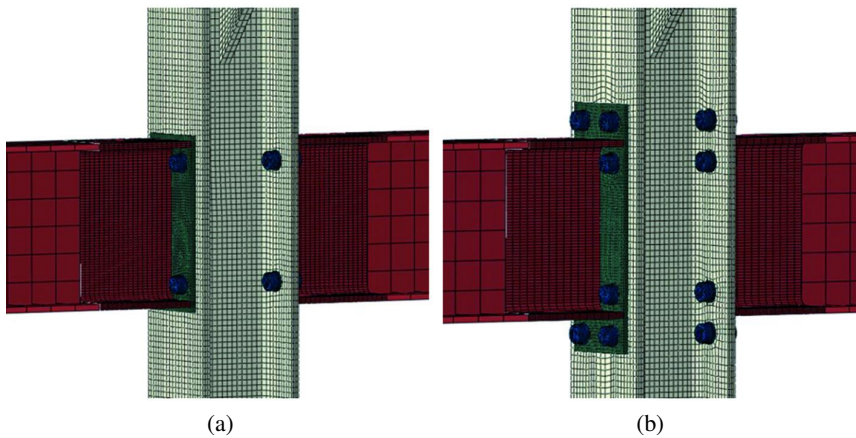
Fig. 5. Detailed view of: a) flush, b) extended end-plate joint with mesh
