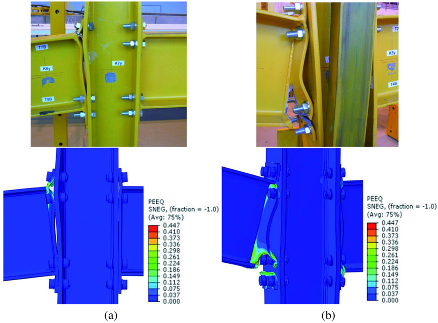
Fig. 8. Failure mode of experimental test [12, 19] and numerical analysis [14] of steel subframe with: a) external column joint, b) internal column joint
