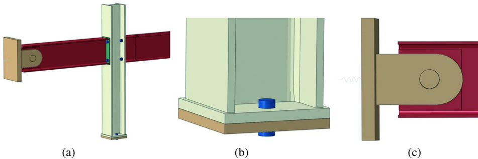
Fig. 4. Detailed view of: a) external column, b) column base, c) external pinned connection
