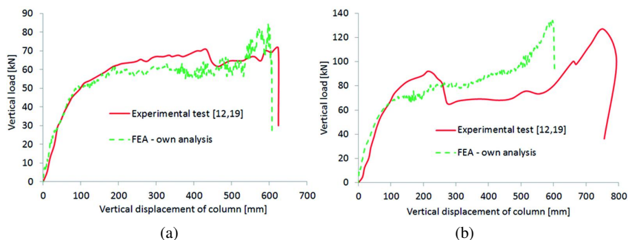
Fig. 6. Response curve load-vertical displacement of specimen with: a) flush end-plate, b) extended end-plate
