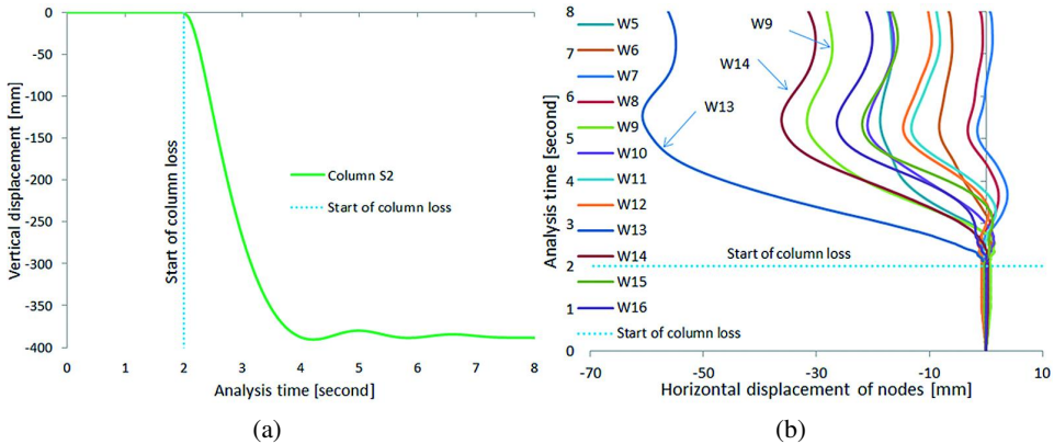
Fig. 11. Curves of: a) vertical displacement – time analysis, b) time analysis vs. horizontal displacement of three bays frame
