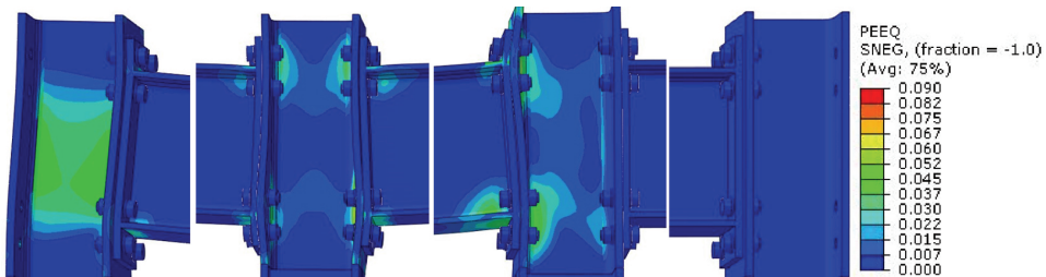
Fig. 15. Map of strains of joint (from left W13 to W16) with 15 mm thickness extended end-plate at level of structure +10.50 at 8 th second of analysis
