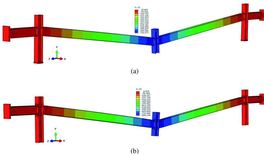
Fig. 7. Map of vertical displacement of model with: a) flush end-plate, b) extended end-plate
