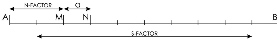
Fig. 5. Sketch of the gradient system showing the position of the electrodes during measurements with the coefficient S = 8 and N = 2 ([36] – modified). AB – supplying electrodes, MN – potential electrodes receiving the current from the medium
