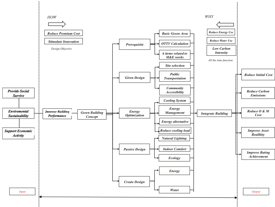
Fig. 2. Function Analysis System Technique Diagram Before Value Engineering
