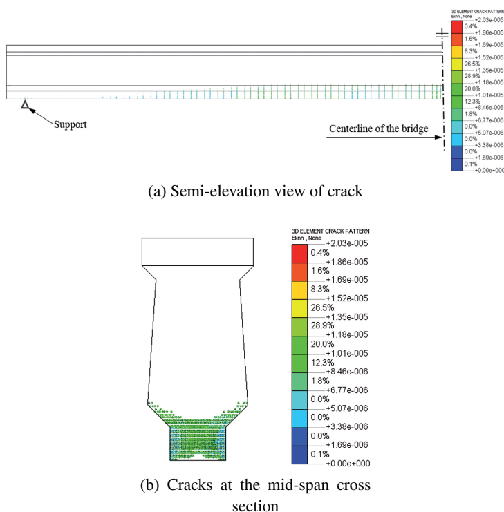
Fig. 17. Cracks distribution of novel joint 1 in stage iv
