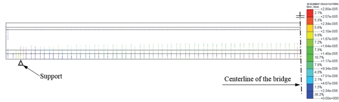
(a) Semi-elevation view of cracks
