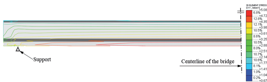
Fig. 8. Semi-elevation view of longitudinal normal stress of J1 (unit: MPa)
