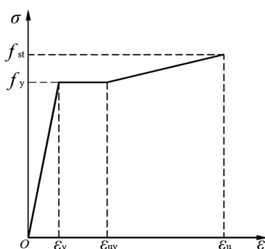
Fig. 14. Ideal elastic-plastic model of steel bar
