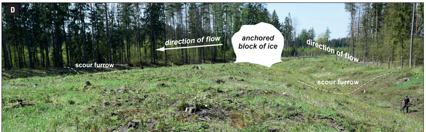
Selected landforms located in the glacial foreland as a result of the Suwałki glacial megaflood: A. the flattened bottom of the Eastern Spillway north of Suwałki, B. a field of giant current ripples formed on the riverbed about 20–24 m deep as a result of the accumulation of sediments carried by the glacial flood south of Suwałki, C. a field of giant current ripples located in the vicinity of Bryzgiel (south of Lake Wigry), D. furrows formed as a result of the scouring flow around a ice block transported by the waters of the glacial flood, which became stranded on the riverbed in the final stage of flooding
