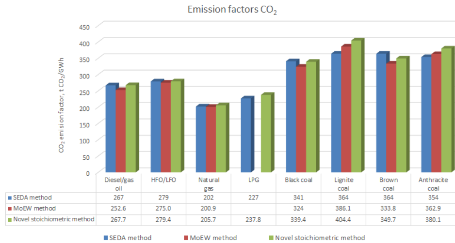
Figure 1: Comparison between the CO 2 emission factors calculated using various methods.
