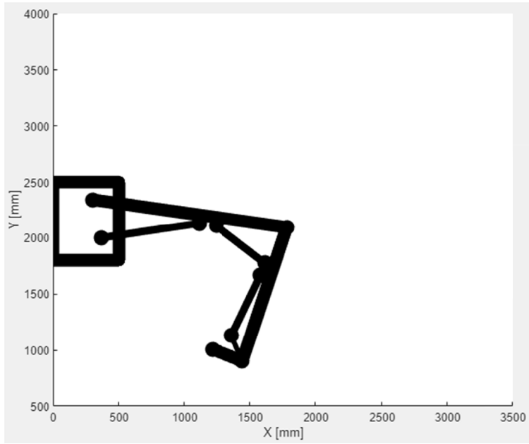
Fig. 8. Movement trajectory of the manipulator tip's movement for the minimal extension of the actuators ( l_{s1} = l_{s2} = l_{s3} = 0 )
