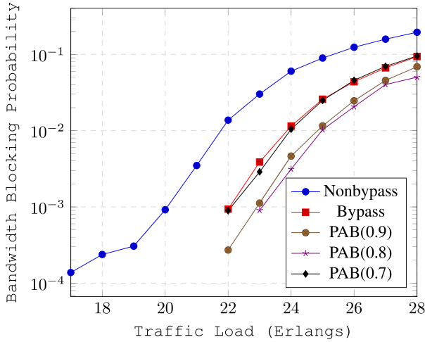
Fig. 9. BBP for overall traffic as a function of the traffic load in the UBN24 network
