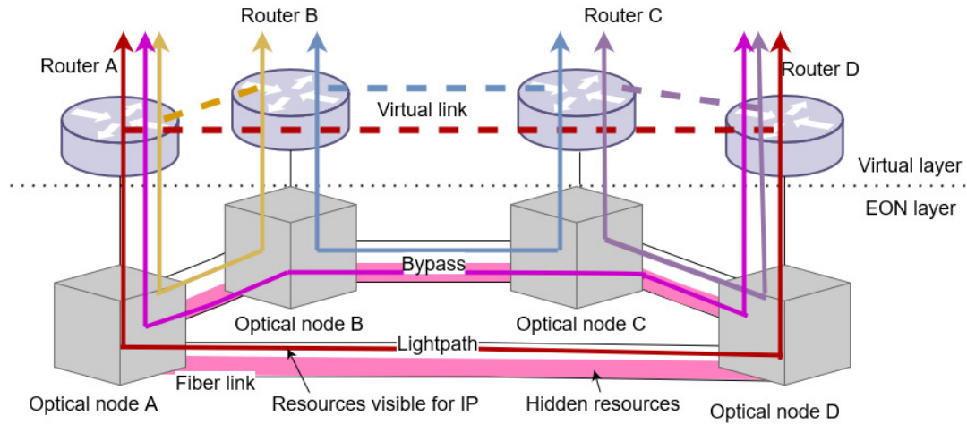
Fig. 1. Example of lightpaths associated with virtual links and bypass
