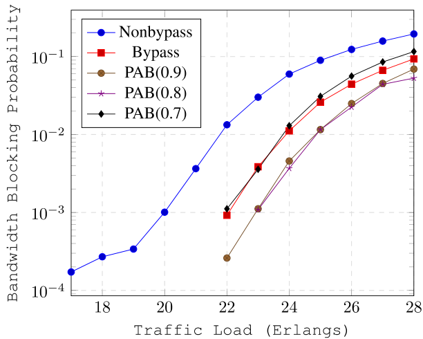
Fig. 13. BBP for low-priority traffic as a function of the traffic load in the UBN24 network
