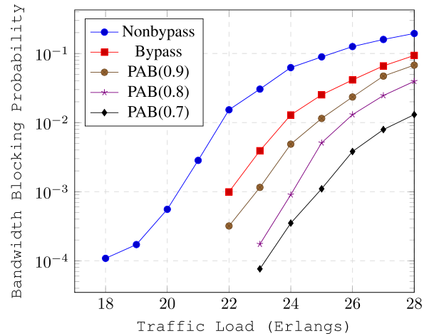
Fig. 11. BBP for high-priority traffic as a function of the traffic load in the UBN24 network
