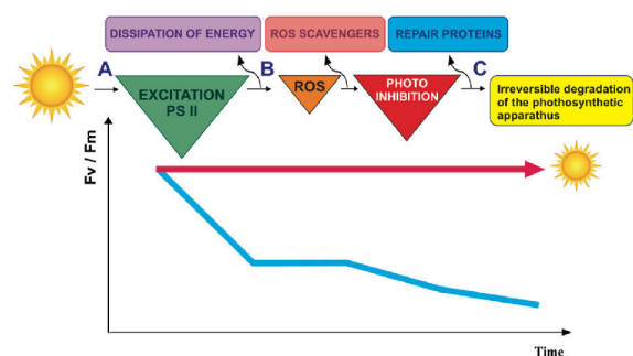
Fig. 6. Graphical interpretation of the changes in photosynthetic activity observed in the lichen study samples. Reduction of Fv/Fm in C. mitis during the culture process - blue line. Physiological changes that occurred in the photosynthetic apparatus: A) activation of photosystem II (PSII), B) formation of reactive oxygen species (ROS), C) irreversible destruction of the photosynthetic apparatus (based on Derks et al., 2015).
