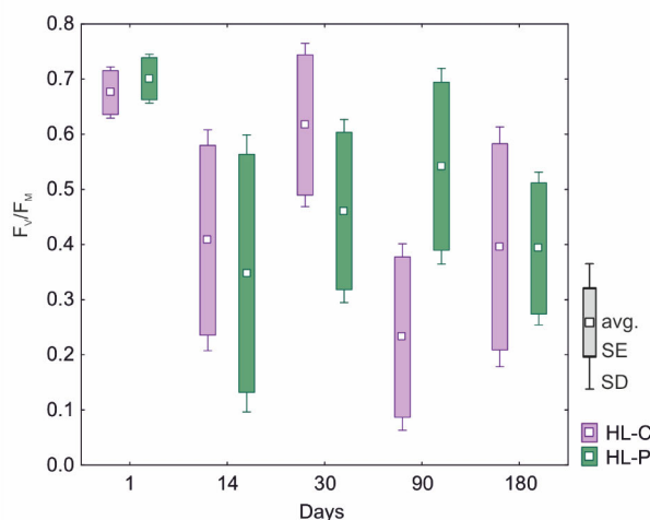
Fig. 4. Mean, \pm SE and SD of the studied lichen and bryophyte species Fv/Fm cultured in HL. The results of ANOVA ( p < 0.05 ) are presented graphically (N=120).
