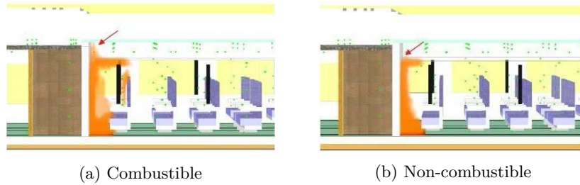
Figure 17: Influence of luggage rack on flame spread.
