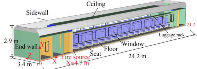
(a) Numerical model of a train fire
