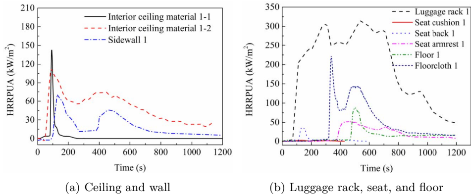
Figure 6: The heat release rate per unit area of each replaced material.
