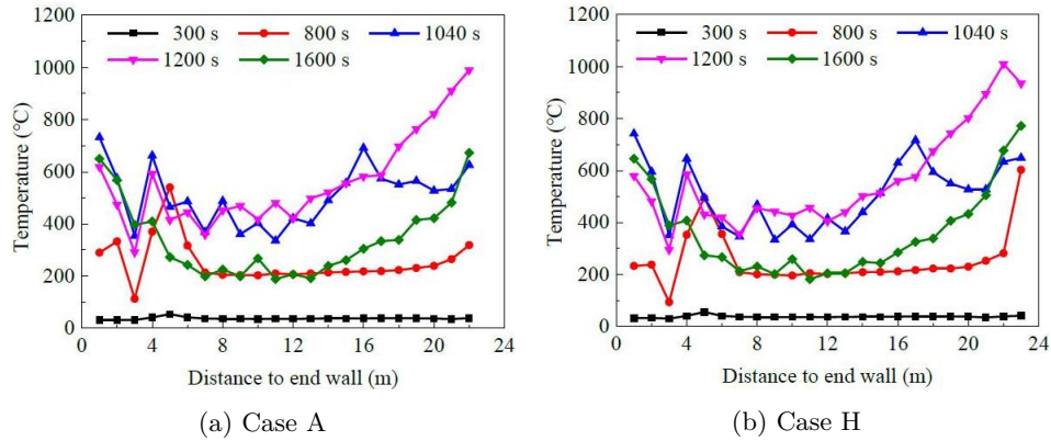
Figure 22: Temperature distribution on the floor surface in the carriage.
