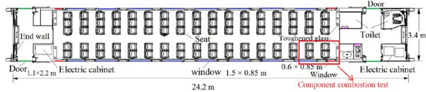
(b) Train carriage plan view
