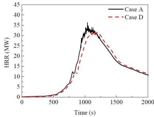
Figure 14: HRR under different sidewall materials.
