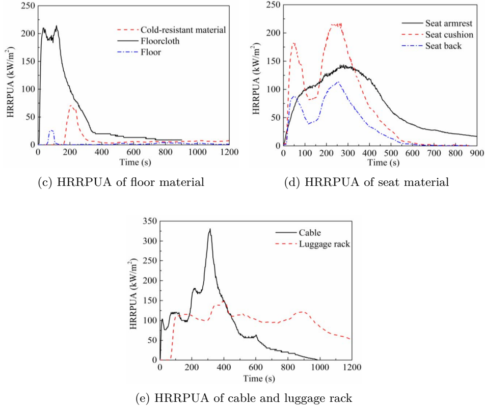
Figure 5: The heat release rate per unit area of different combustible materials in the train carriage.
