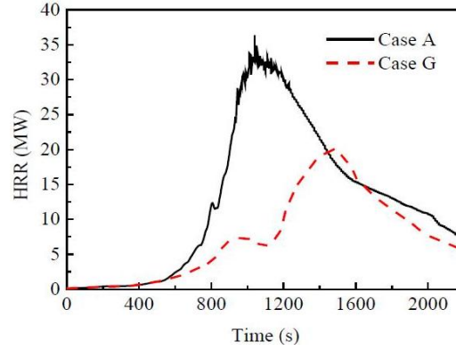
Figure 18: HRR under different seat materials.
