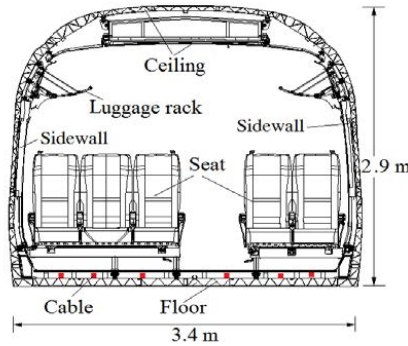
(a) Train carriage sectional view
