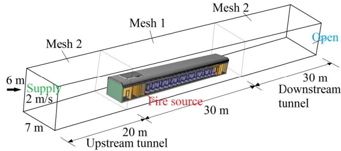
(b) Computational domain of the numerical model
