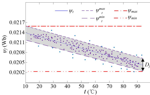
Fig. 3. Distribution of \psi_f initialization.
