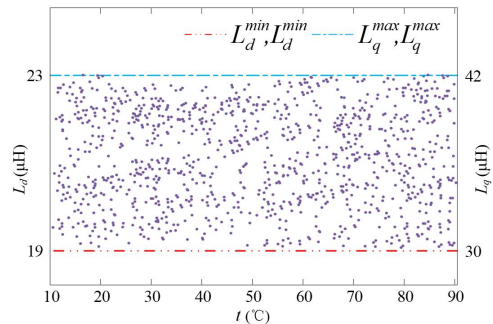
Fig. 4. Distribution of L_d and L_q initialization.
