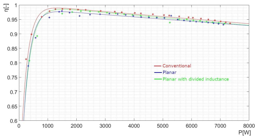
Fig. 9. Efficiency characteristics obtained
