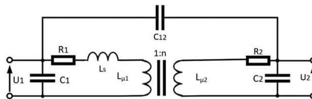
Fig. 5. Equivalent diagram of a transformer
