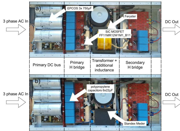
Fig. 6. View of tested system
