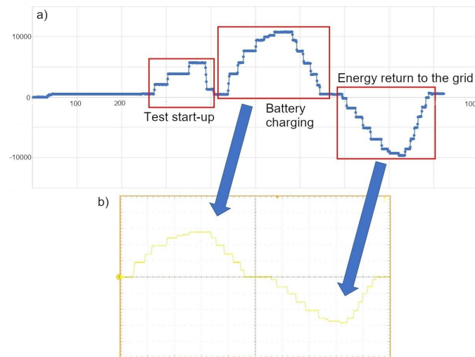
Fig. 14. Input power (a) and output current waveforms (b) of the charging system
