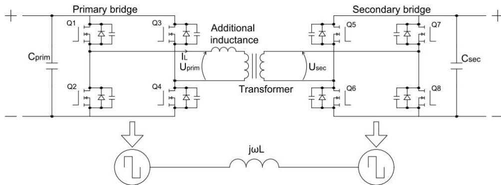
Fig. 7. Diagram of tested system
