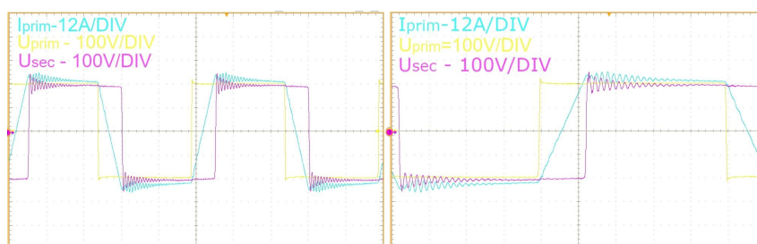
Fig. 10. Voltage and current waveforms on the primary and secondary side in the planar transformer circuit for phase shift \varphi = 45^\circ
