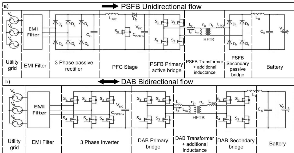
Fig. 2. Diagram of an electric vehicle charging station: (a) one-way PSFB; (b) two-way DAB
