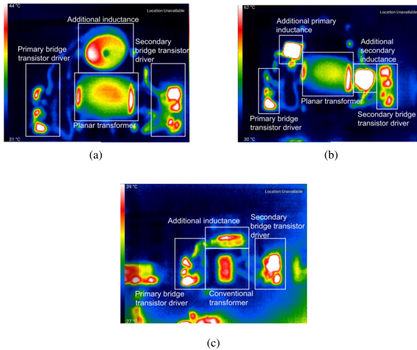
Fig. 13. Thermal images on 7.3 kW load for: (a) planar transformer; (b) planar transformer with divided additional inductance; (c) conventional transformer
