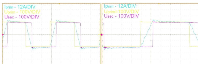
Fig. 11. Voltage and current waveforms on the primary and secondary side in the planar transformer circuit with divided additional inductance for phase shift \varphi = 45^\circ
