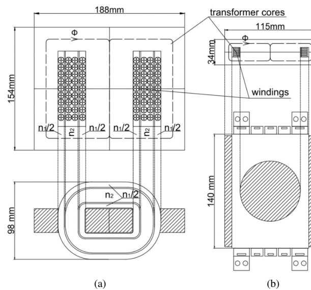
Fig. 4. Cross-section of a planar and a conventional transformer
