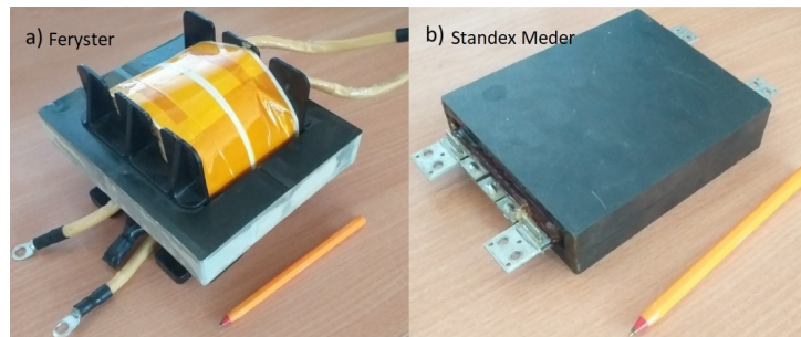
Fig. 3. Transformers examined: (a) conventional Feryster transformer; (b) Standex Meder planar transformer
