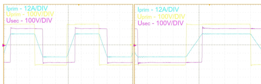
Fig. 12. Voltage and current waveforms on the primary and secondary side in the conventional transformer circuit for phase shift \varphi = 45^\circ
