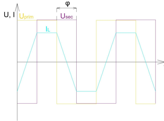
Fig. 8. The voltage and current waveforms of the system under test
