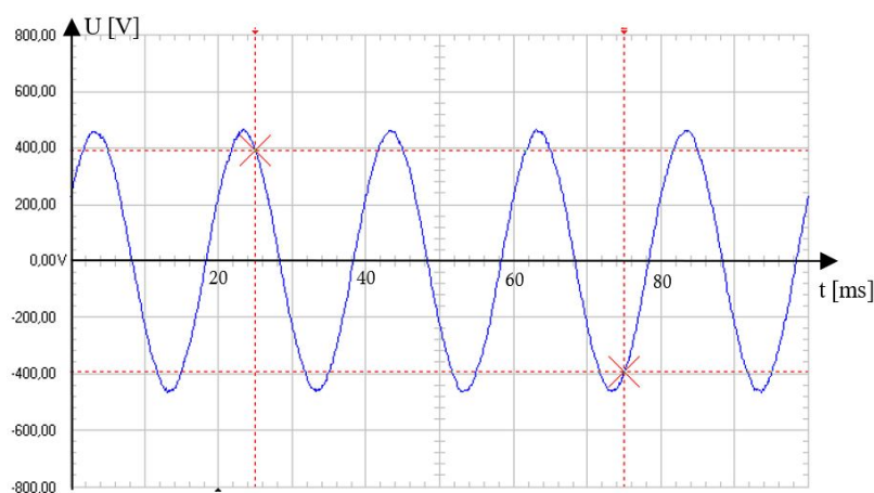
Fig. 12. Waveform at the output of induction machine with PCW from side 2p = 6
