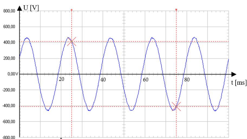
Fig. 13. Waveform at the output of induction machine with PCW from side 2p = 8
