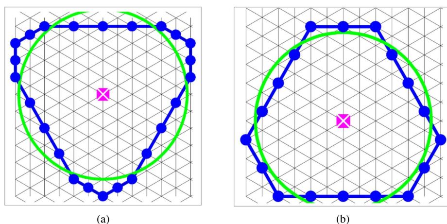
Fig. 7. Görges polygons of DSSF: (a) 6-pole winding with \sigma_d = 4.16\% and \xi = 0.872 ; (b) 8-pole winding with \sigma_d = 2.18\% and \xi = 0.819
