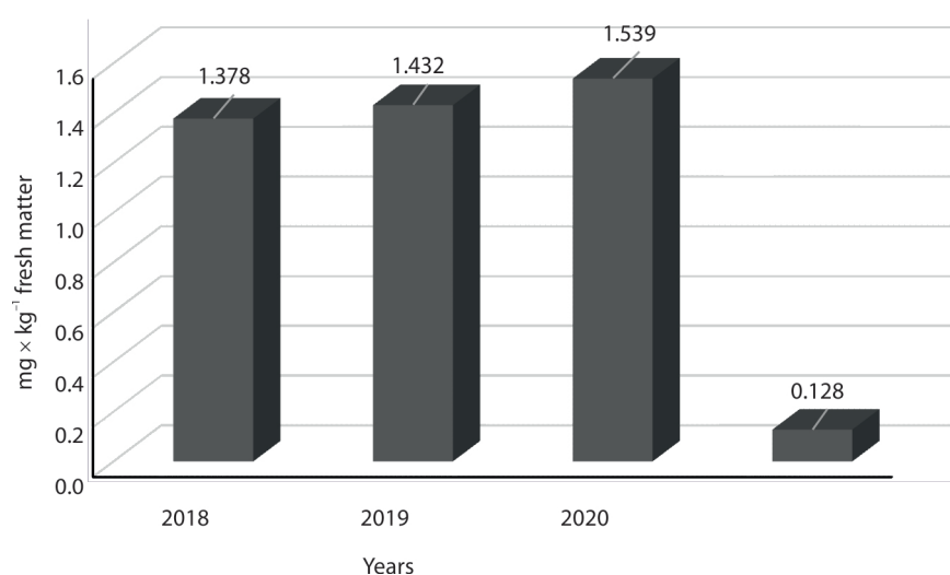
Fig. 3. Content of total carotenoids in potato tubers ( \text{mg} \times \text{kg}^{-1} fresh matter) depending on the year of study
