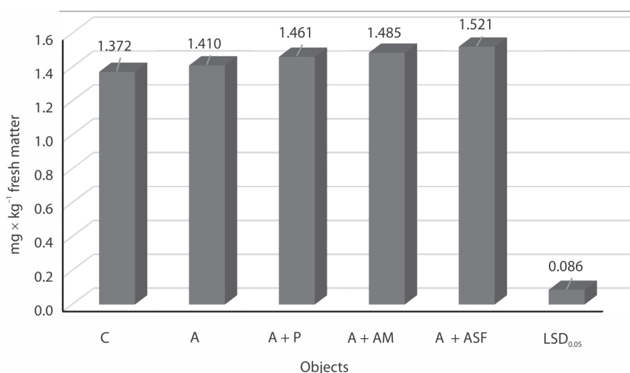
Fig. 2. Content of total carotenoids in potato tubers ( \text{mg} \times \text{kg}^{-1} fresh matter) depending on biostimulants and herbicide C – control object; A – Avatar 293 ZC; A + P – Avatar 293 ZC + PlonoStart A + AM – Avatar 293 ZC + Aminoplant; A + ASF – Avatar 293 ZC + Agro Sorb Folium
