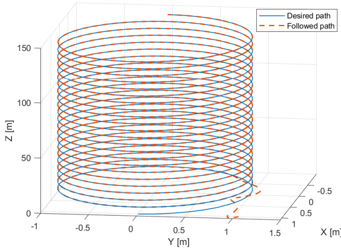
Figure 6: The desired path \alpha(s) and the path followed by the RTR manipulator for k_k = 10 , k_d = 30 , \gamma = 100
