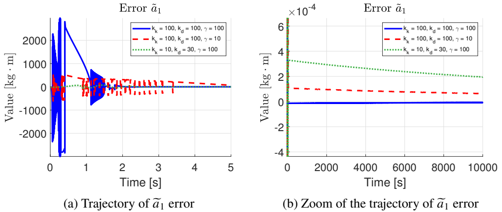
Figure 15: Estimation error \tilde{a}_1 for the tapering helix \beta(u) (Solid line: k_k = 100 , k_d = 100 , \gamma = 100 ; Dashed line: k_k = 100 , k_d = 100 , \gamma = 10 ; Dotted line: k_k = 10 , k_d = 30 , \gamma = 100 )
