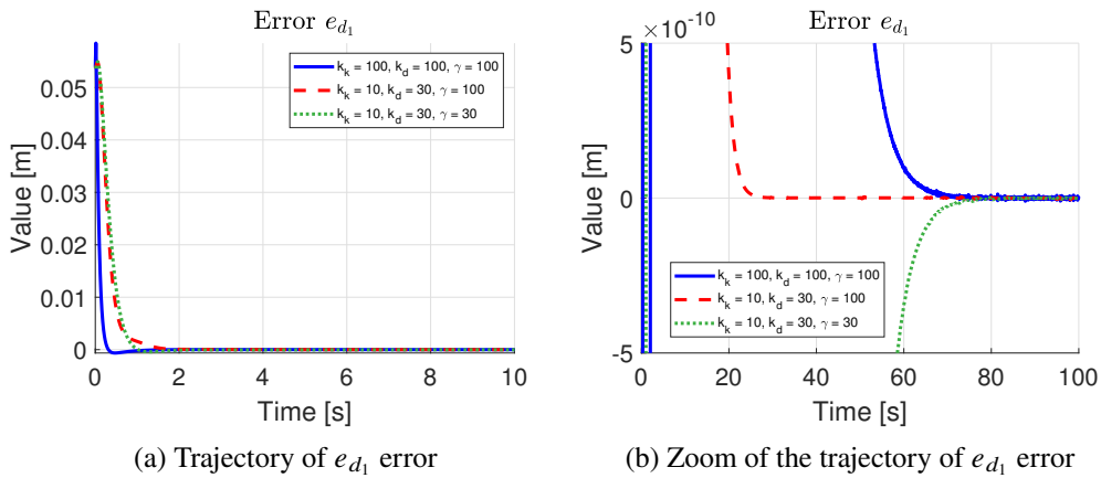
Figure 18: Path following error e_{d1} for the helix \alpha(s) – RX-60 manipulator (Solid line: k_k = 100 , k_d = 100 , \gamma = 100 ; Dashed line: k_k = 10 , k_d = 30 , \gamma = 100 ; Dotted line: k_k = 10 , k_d = 30 , \gamma = 30 )
