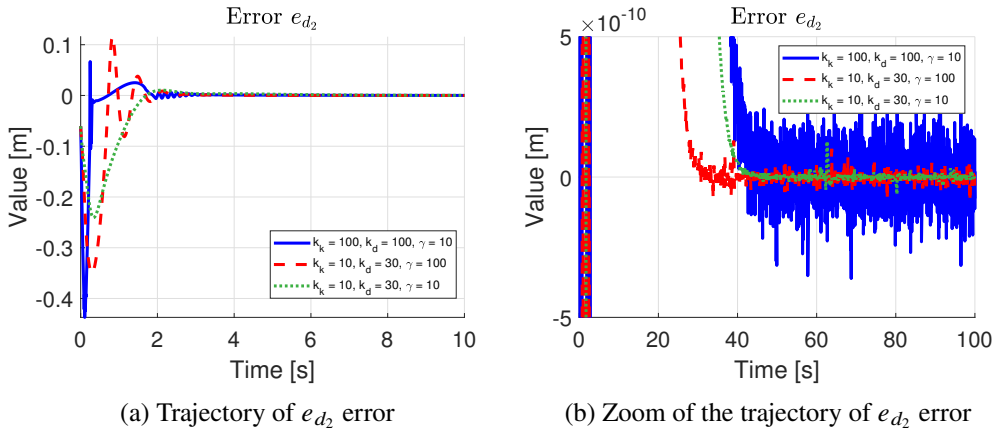
Figure 8: Path following error e_{d2} for the helix \alpha(s) – RTR manipulator (Solid line: k_k = 100, k_d = 100, \gamma = 10 ; Dashed line: k_k = 10, k_d = 30, \gamma = 100 ; Dotted line: k_k = 10, k_d = 30, \gamma = 10 )
