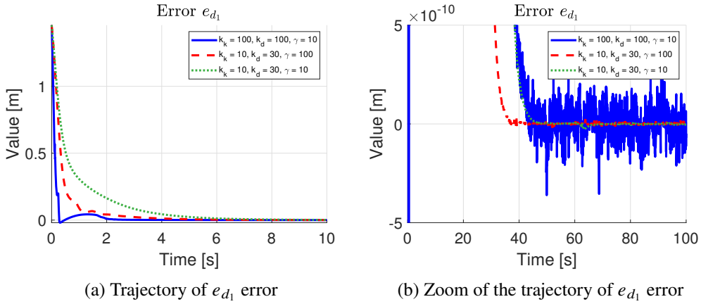
Figure 7: Path following error e_{d1} for the helix \alpha(s) – RTR manipulator (Solid line: k_k = 100, k_d = 100, \gamma = 10 ; Dashed line: k_k = 10, k_d = 30, \gamma = 100 ; Dotted line: k_k = 10, k_d = 30, \gamma = 10 )
