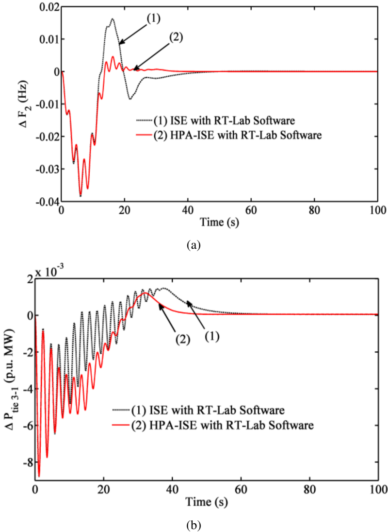
Figure 9: System dynamics with HPA-ISE and ISE: (a) \Delta F_2 and (b) \Delta P_{31} in RT-lab
