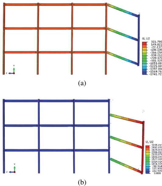
Fig. 5. Map of vertical displacement of case 4B_F15 under selected time of analysis: a) 3.5 th second, b) 5 th second
