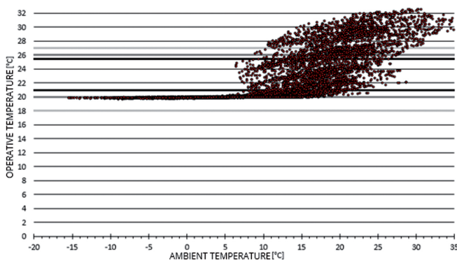
Fig. 1. Dependence of the operative temperature on the ambient temperature
