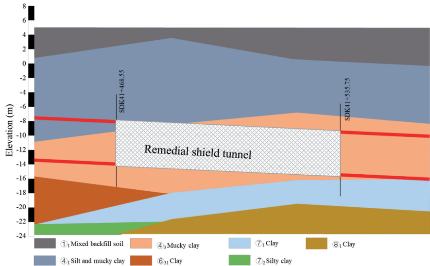
Fig. 2. (Color) Partial longitudinal geological profile of the up-track tunnel
