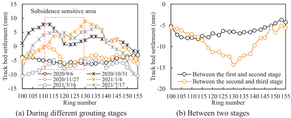
Fig. 13. Track bed settlement under different grouting stages
