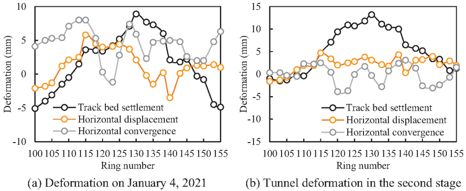
Fig. 10. Variation of the tunnel deformation caused by the second stage grouting
