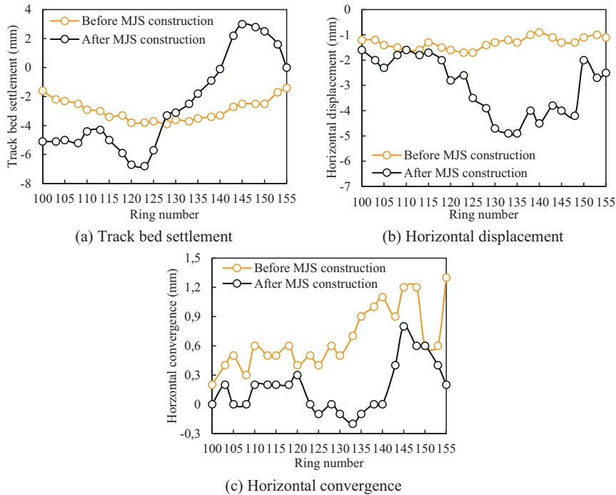
Fig. 8. Comparison results of damaged TBM tunnel deformation
