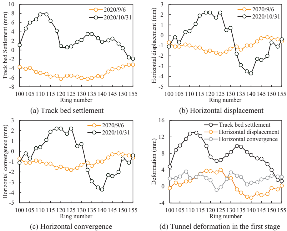
Fig. 9. Comparison results of damaged TBM tunnel deformation
