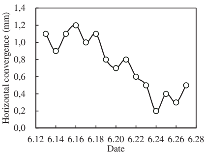
(c) Horizontal convergence
