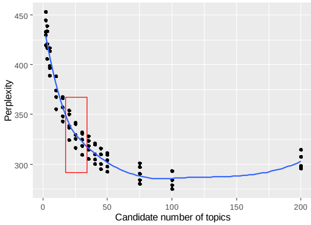
Fig. 2. Result of perplexity computation for MS. The trend line is in blue. Acceptable k -interval between 20 and 30 is highlighted in red, where the trend line bends
