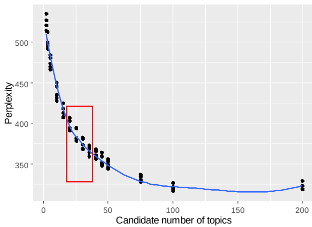
Fig. 4. Result of perplexity computation for OM. The trend line is in blue. Acceptable k -interval between 20 and 35 is highlighted in red, where the trend line bends
