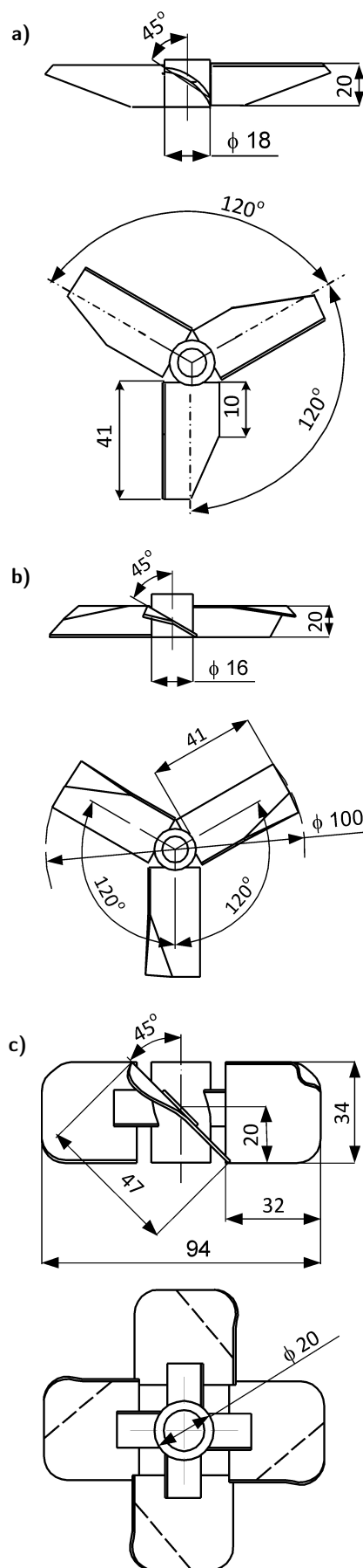
Figure 2. Impellers: a) SC-3, b) HE-3, c) A315.
